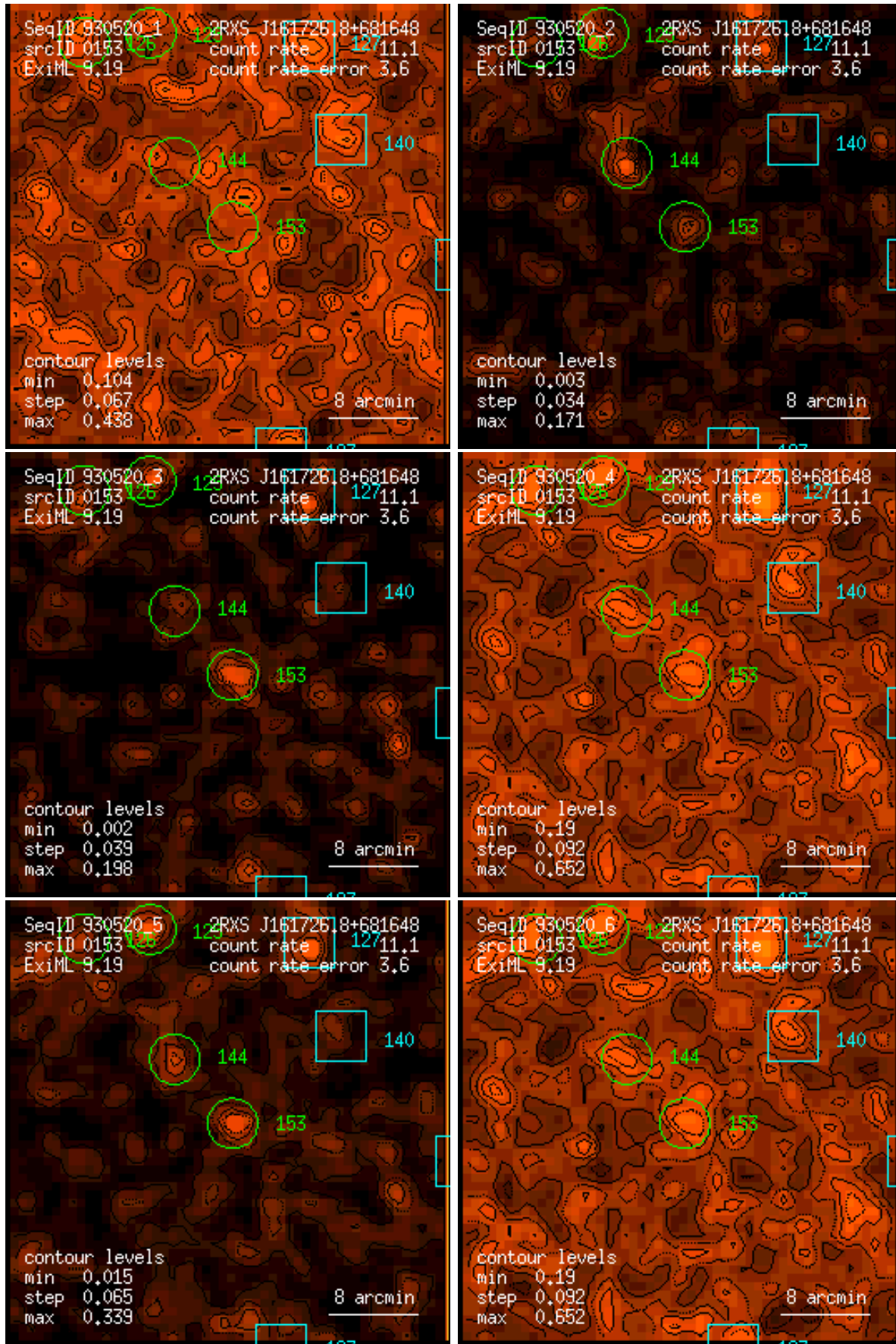
Figure 153: RASS 930520: detection 0153: band rate images, Gaussian filter: (1) PSPC channels 11 – 41, (2) 52 – 90, (3) 91 – 201, (4) 11 – 235, (5) 52 – 201, (6) 11 – 201. Broad band rates in counts/ks. Band rate contour levels in counts/ks/arcmin 2 .
