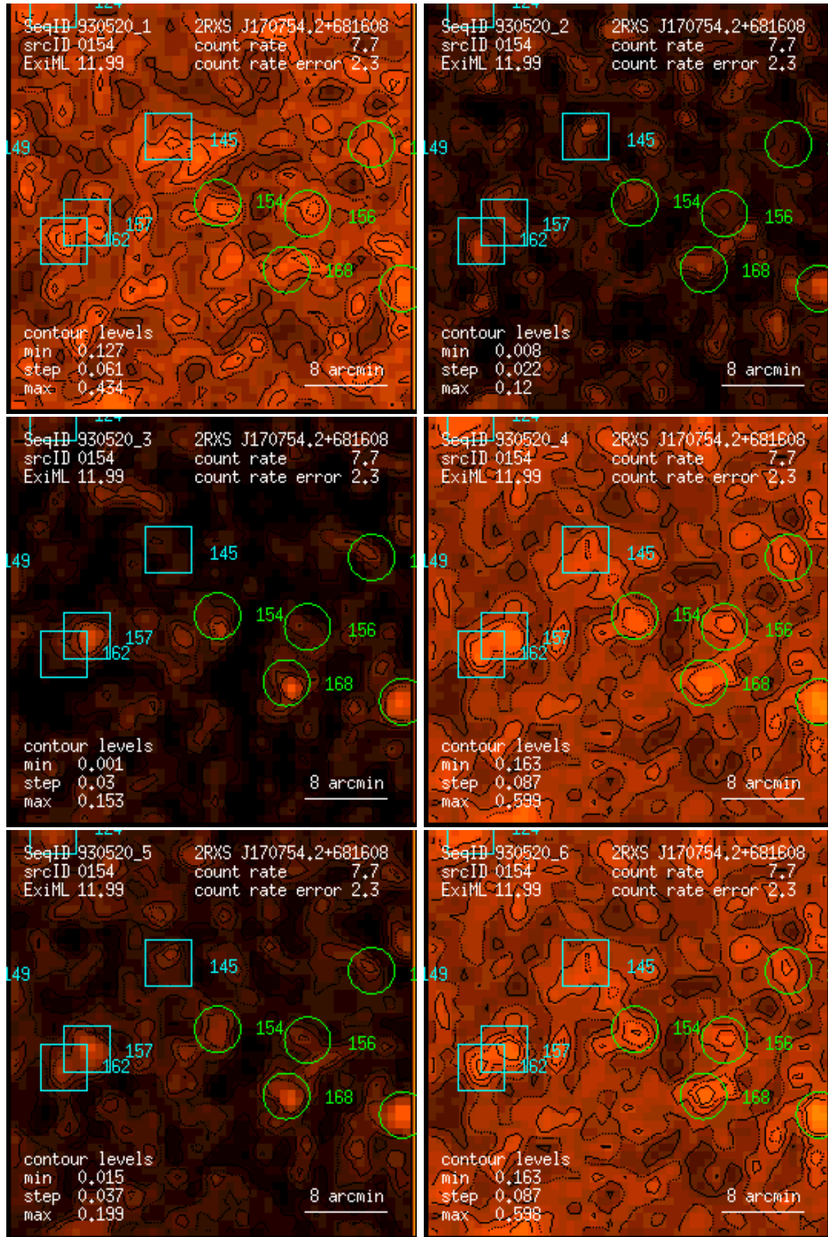
Figure 154: RASS 930520: detection 0154: band rate images, Gaussian filter: (1) PSPC channels 11 – 41, (2) 52 – 90, (3) 91 – 201, (4) 11 – 235, (5) 52 – 201, (6) 11 – 201. Broad band rates in counts/ks. Band rate contour levels in counts/ks/arcmin 2 .
