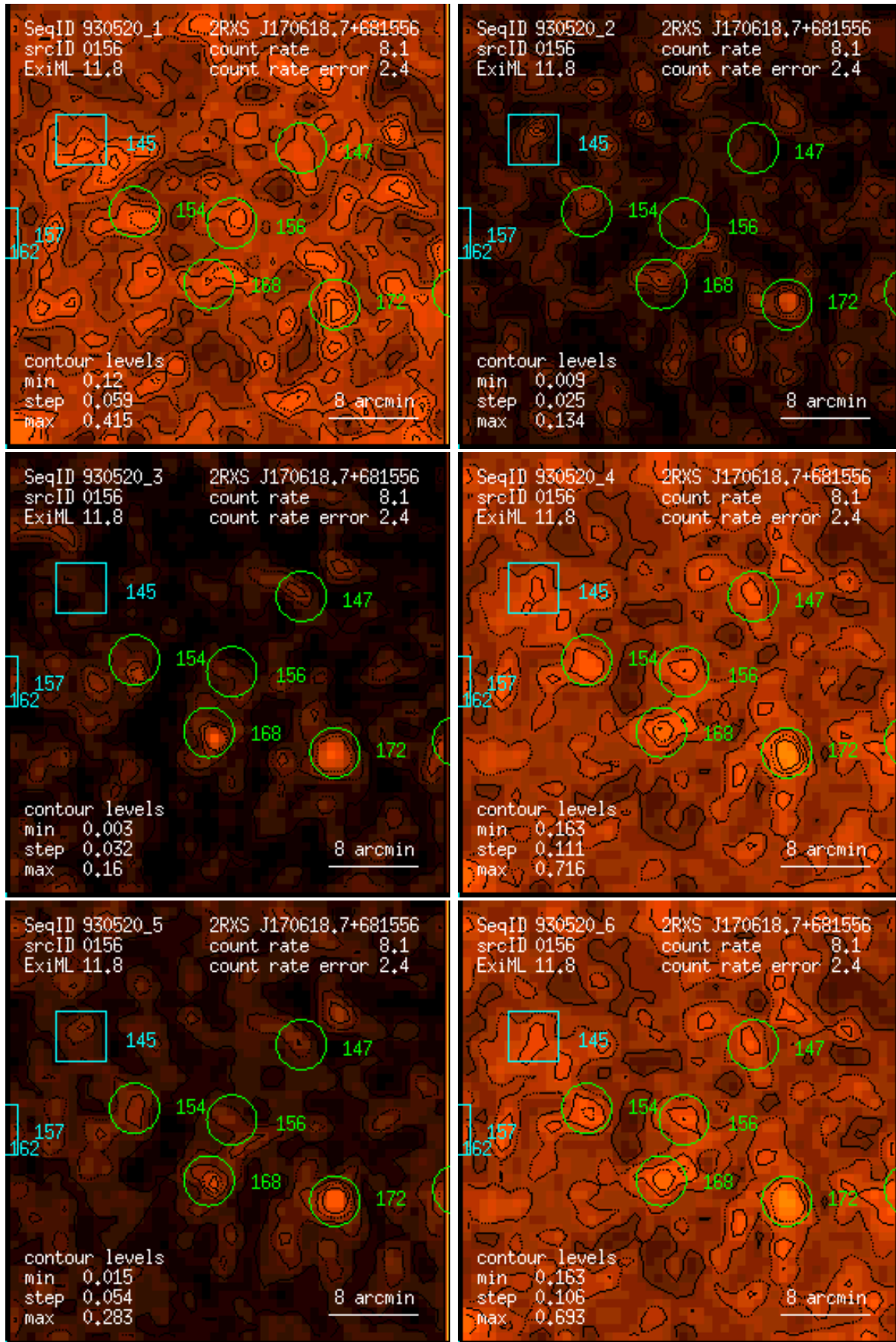
Figure 156: RASS 930520: detection 0156: band rate images, Gaussian filter: (1) PSPC channels 11 – 41, (2) 52 – 90, (3) 91 – 201, (4) 11 – 235, (5) 52 – 201, (6) 11 – 201. Broad band rates in counts/ks. Band rate contour levels in counts/ks/arcmin 2 .
