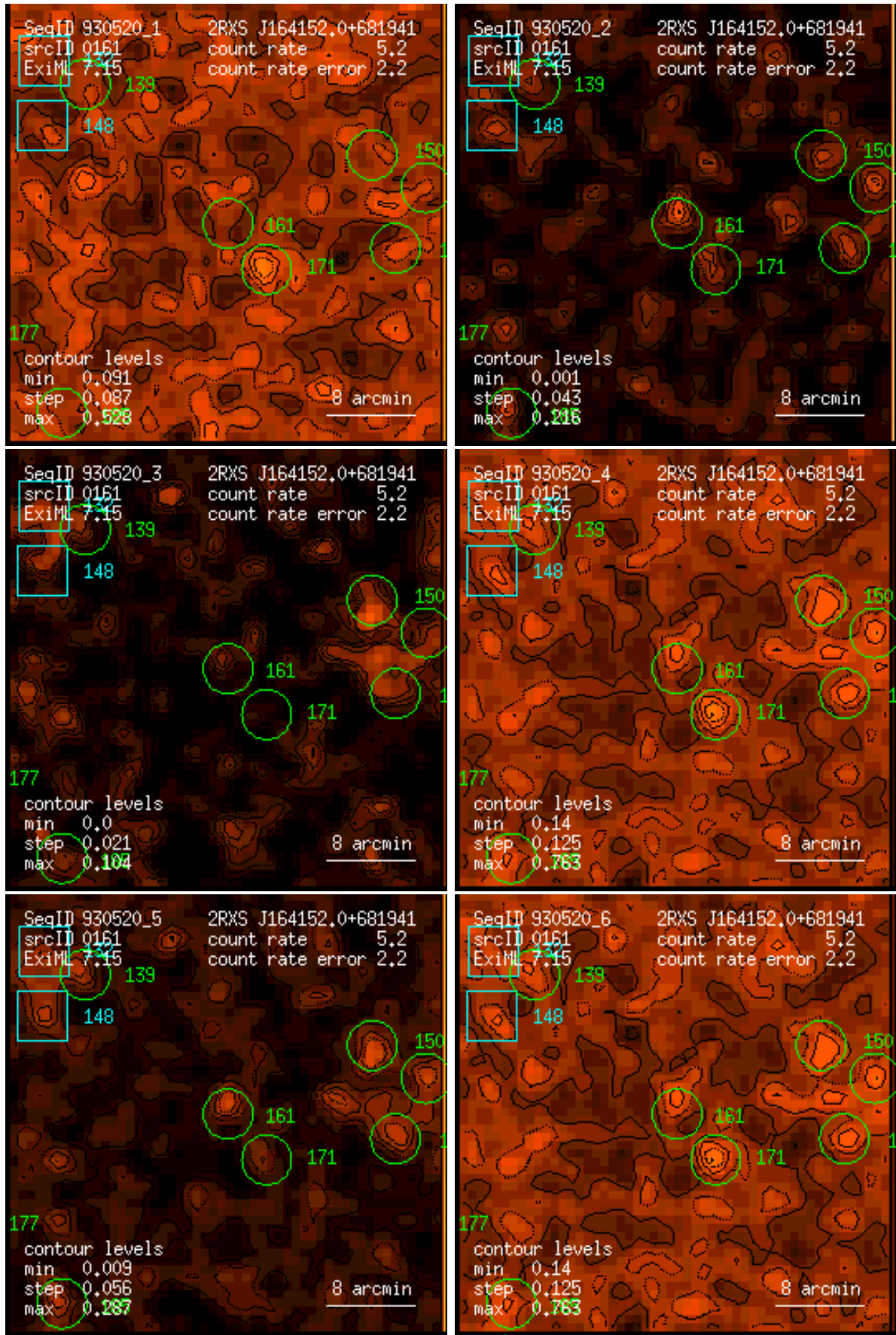
Figure 161: RASS 930520: detection 0161: band rate images, Gaussian filter: (1) PSPC channels 11 – 41, (2) 52 – 90, (3) 91 – 201, (4) 11 – 235, (5) 52 – 201, (6) 11 – 201. Broad band rates in counts/ks. Band rate contour levels in counts/ks/arcmin 2 .
