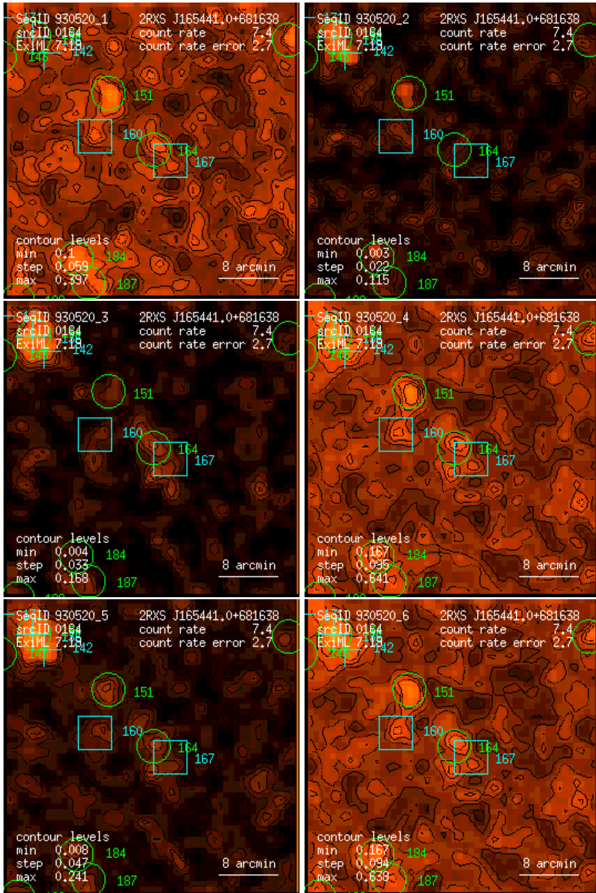
Figure 164: RASS 930520: detection 0164: band rate images, Gaussian filter: (1) PSPC channels 11 – 41, (2) 52 – 90, (3) 91 – 201, (4) 11 – 235, (5) 52 – 201, (6) 11 – 201. Broad band rates in counts/ks. Band rate contour levels in counts/ks/arcmin 2 .
