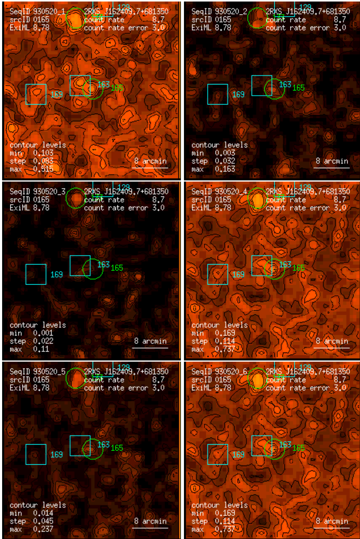
Figure 165: RASS 930520: detection 0165: band rate images, Gaussian filter: (1) PSPC channels 11 – 41, (2) 52 – 90, (3) 91 – 201, (4) 11 – 235, (5) 52 – 201, (6) 11 – 201. Broad band rates in counts/ks. Band rate contour levels in counts/ks/arcmin 2 .
