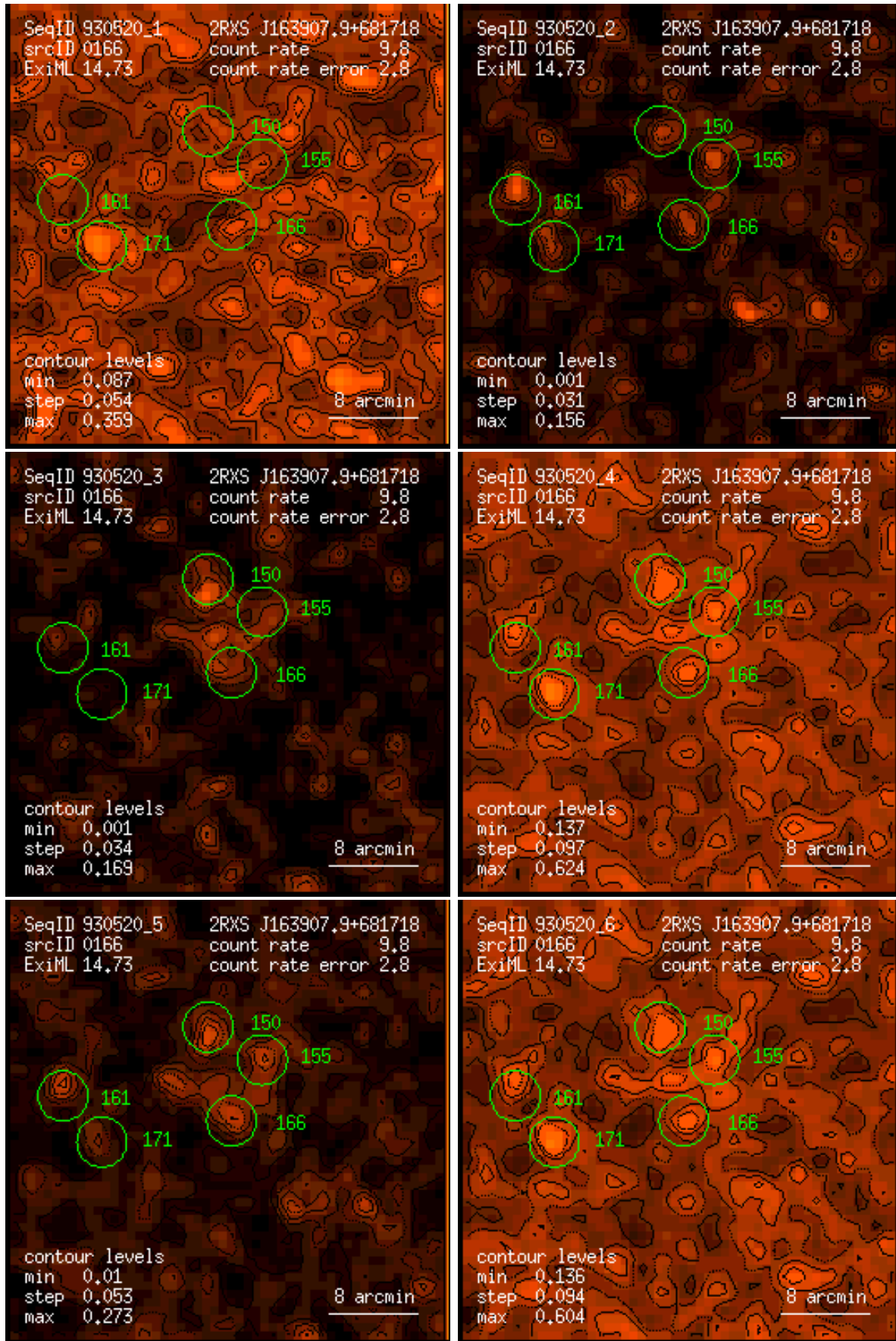
Figure 166: RASS 930520: detection 0166: band rate images, Gaussian filter: (1) PSPC channels 11 – 41, (2) 52 – 90, (3) 91 – 201, (4) 11 – 235, (5) 52 – 201, (6) 11 – 201. Broad band rates in counts/ks. Band rate contour levels in counts/ks/arcmin 2 .
