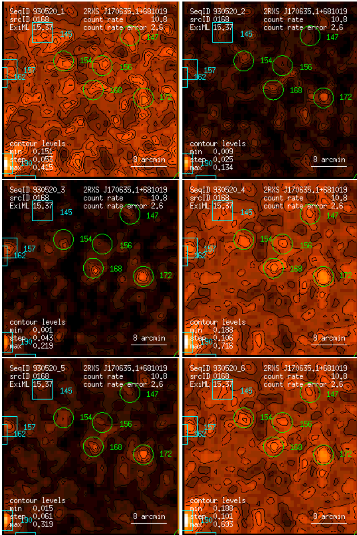
Figure 168: RASS 930520: detection 0168: band rate images, Gaussian filter: (1) PSPC channels 11 – 41, (2) 52 – 90, (3) 91 – 201, (4) 11 – 235, (5) 52 – 201, (6) 11 – 201. Broad band rates in counts/ks. Band rate contour levels in counts/ks/arcmin 2 .
