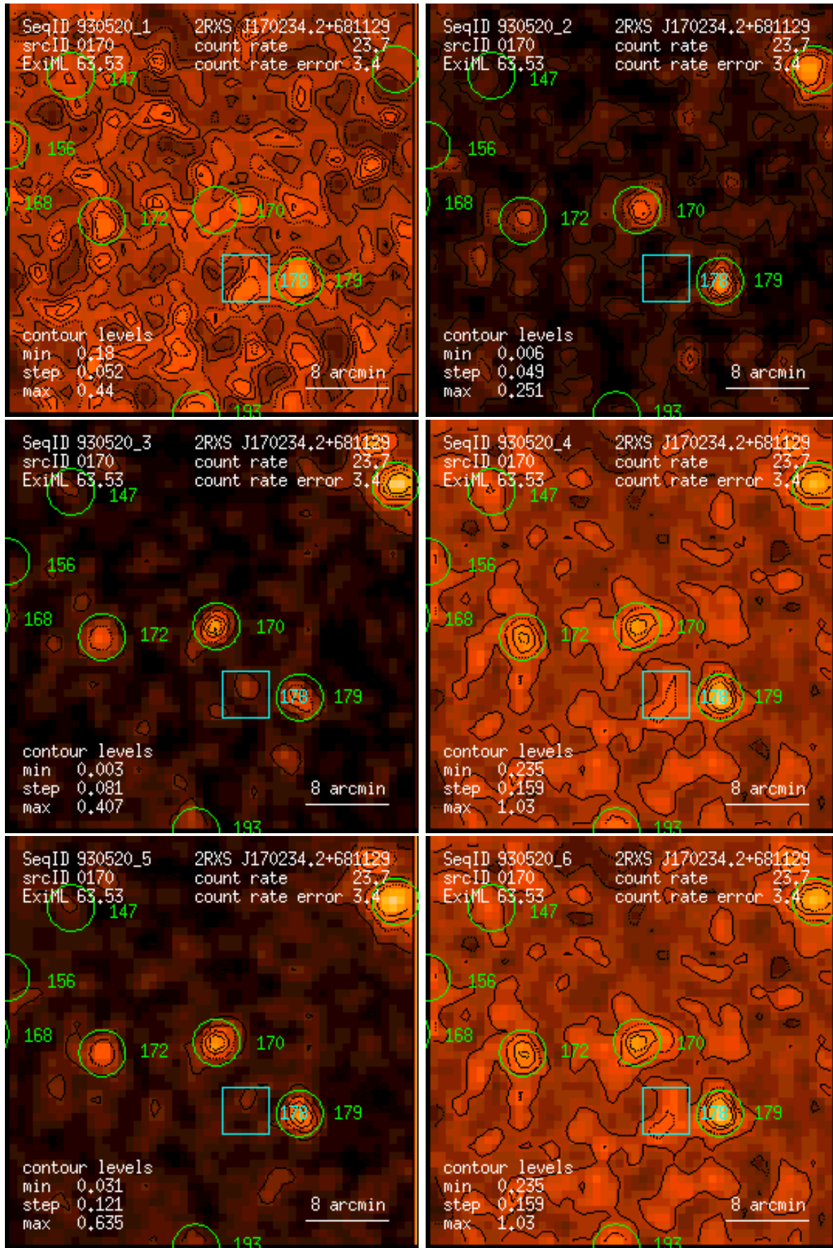
Figure 170: RASS 930520: detection 0170: band rate images, Gaussian filter: (1) PSPC channels 11 – 41, (2) 52 – 90, (3) 91 – 201, (4) 11 – 235, (5) 52 – 201, (6) 11 – 201. Broad band rates in counts/ks. Band rate contour levels in counts/ks/arcmin 2 .
