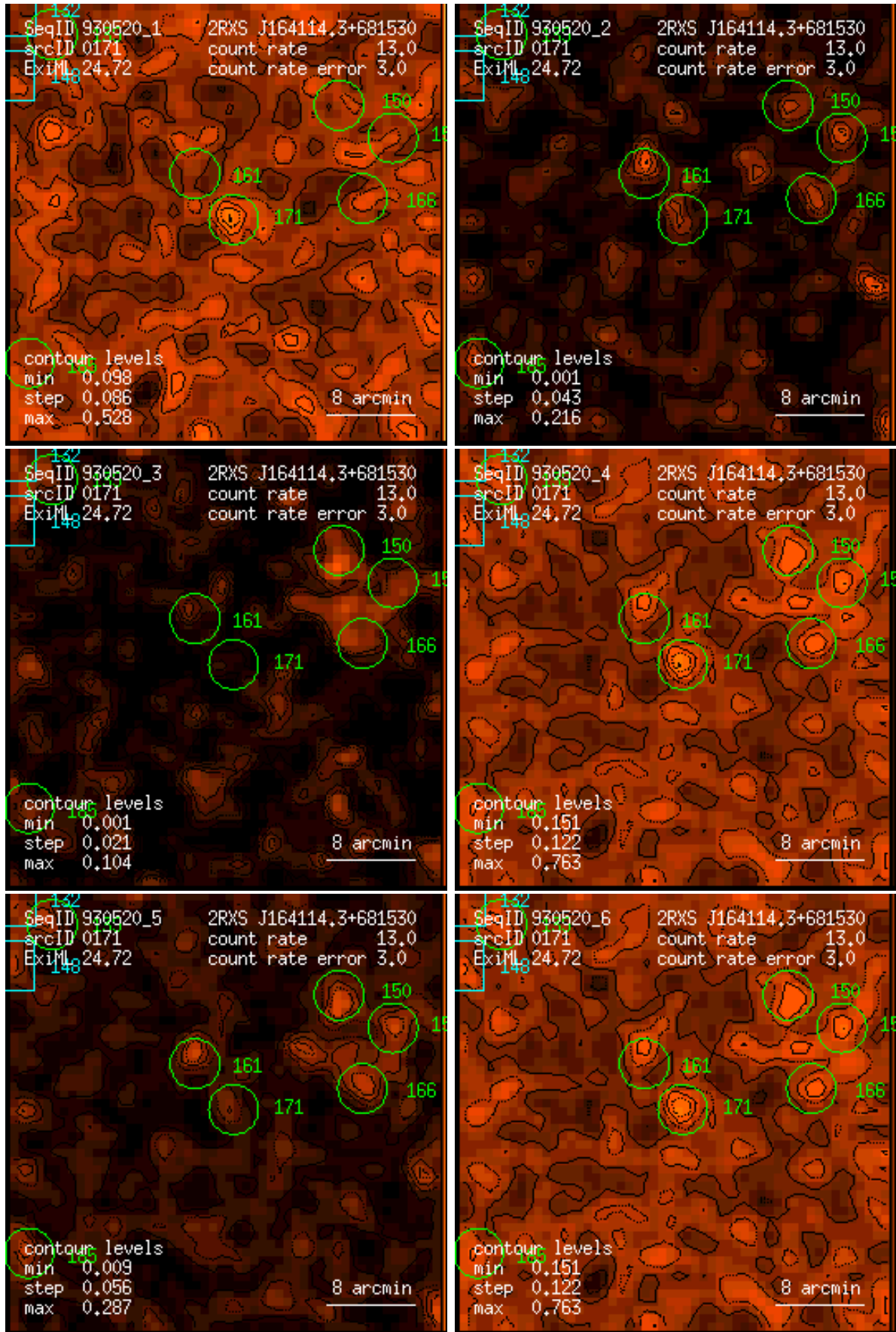
Figure 171: RASS 930520: detection 0171: band rate images, Gaussian filter: (1) PSPC channels 11 – 41, (2) 52 – 90, (3) 91 – 201, (4) 11 – 235, (5) 52 – 201, (6) 11 – 201. Broad band rates in counts/ks. Band rate contour levels in counts/ks/arcmin 2 .
