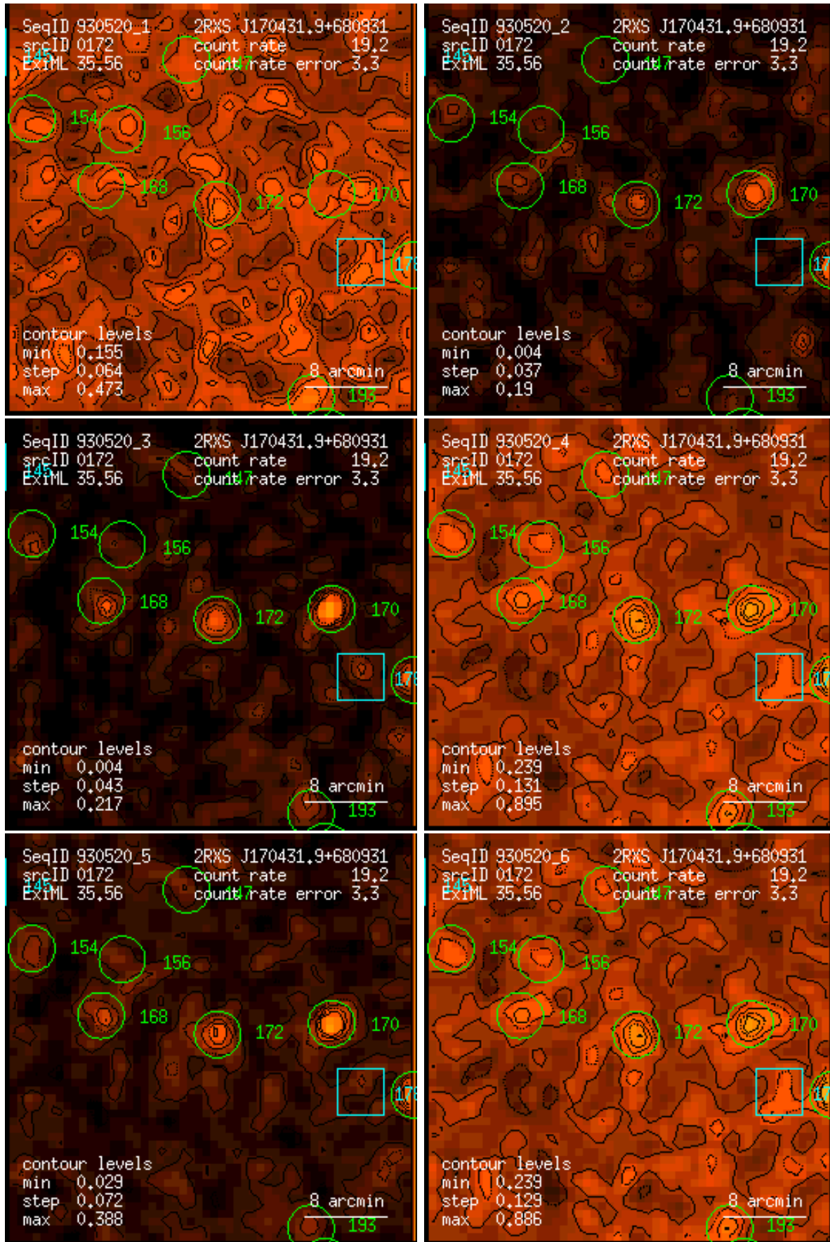
Figure 172: RASS 930520: detection 0172: band rate images, Gaussian filter: (1) PSPC channels 11 – 41, (2) 52 – 90, (3) 91 – 201, (4) 11 – 235, (5) 52 – 201, (6) 11 – 201. Broad band rates in counts/ks. Band rate contour levels in counts/ks/arcmin 2 .
