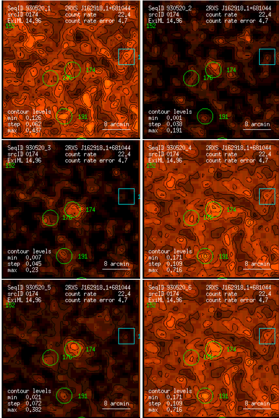
Figure 174: RASS 930520: detection 0174: band rate images, Gaussian filter: (1) PSPC channels 11 – 41, (2) 52 – 90, (3) 91 – 201, (4) 11 – 235, (5) 52 – 201, (6) 11 – 201. Broad band rates in counts/ks. Band rate contour levels in counts/ks/arcmin 2 .
