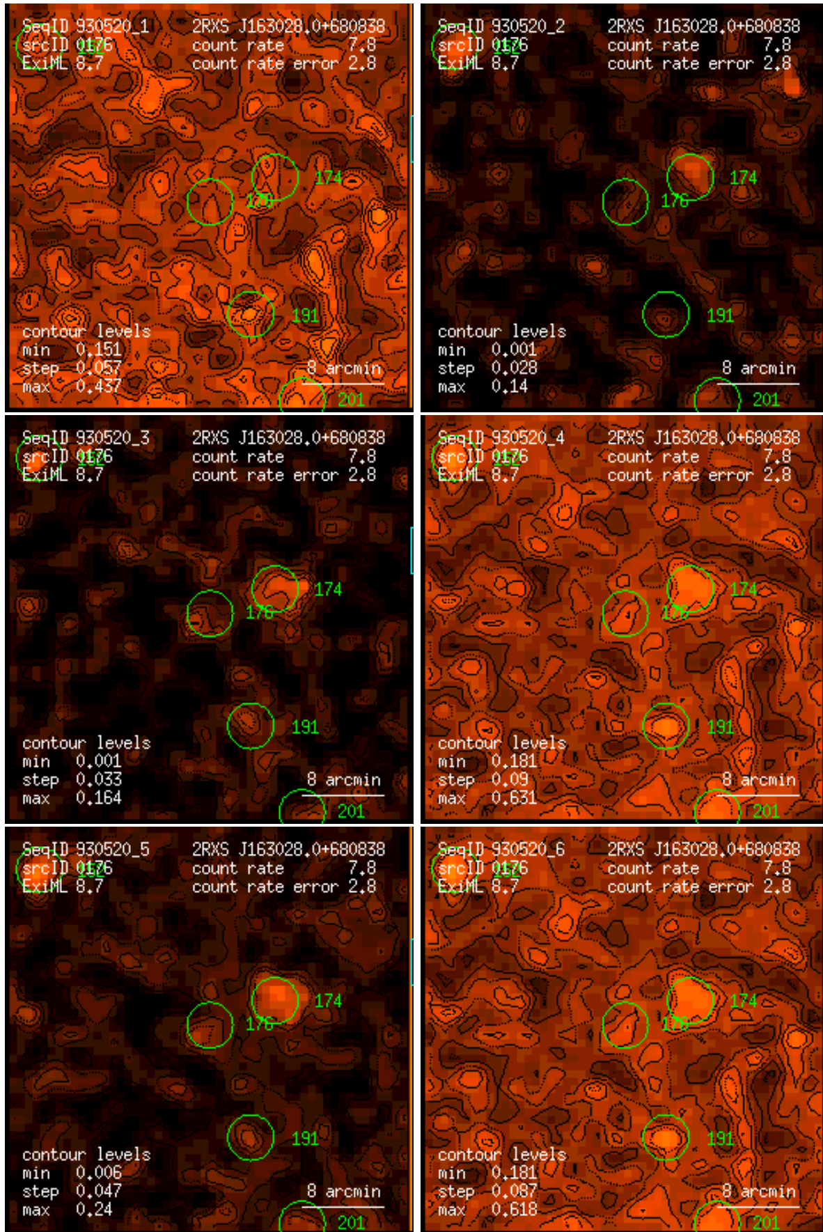
Figure 176: RASS 930520: detection 0176: band rate images, Gaussian filter: (1) PSPC channels 11 – 41, (2) 52 – 90, (3) 91 – 201, (4) 11 – 235, (5) 52 – 201, (6) 11 – 201. Broad band rates in counts/ks. Band rate contour levels in counts/ks/arcmin 2 .
