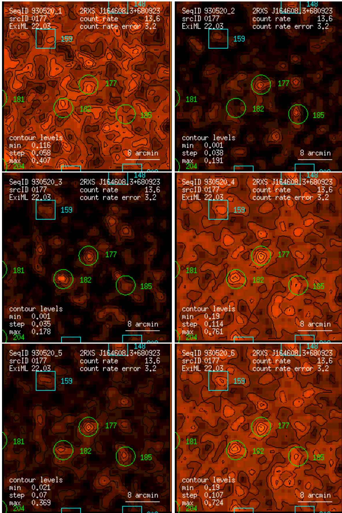
Figure 177: RASS 930520: detection 0177: band rate images, Gaussian filter: (1) PSPC channels 11 – 41, (2) 52 – 90, (3) 91 – 201, (4) 11 – 235, (5) 52 – 201, (6) 11 – 201. Broad band rates in counts/ks. Band rate contour levels in counts/ks/arcmin 2 .
