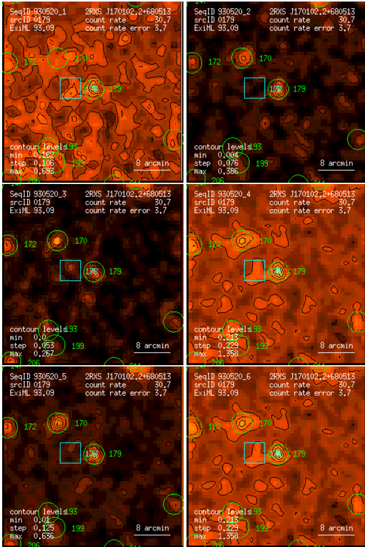
Figure 179: RASS 930520: detection 0179: band rate images, Gaussian filter: (1) PSPC channels 11 – 41, (2) 52 – 90, (3) 91 – 201, (4) 11 – 235, (5) 52 – 201, (6) 11 – 201. Broad band rates in counts/ks. Band rate contour levels in counts/ks/arcmin 2 .
