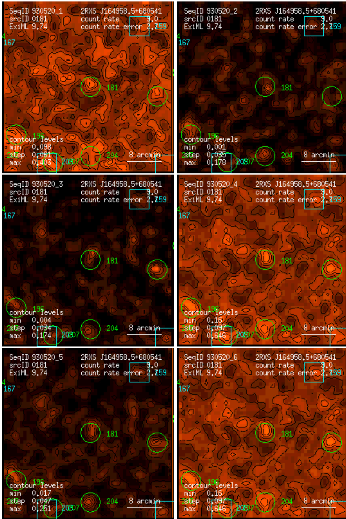
Figure 181: RASS 930520: detection 0181: band rate images, Gaussian filter: (1) PSPC channels 11 – 41, (2) 52 – 90, (3) 91 – 201, (4) 11 – 235, (5) 52 – 201, (6) 11 – 201. Broad band rates in counts/ks. Band rate contour levels in counts/ks/arcmin 2 .
