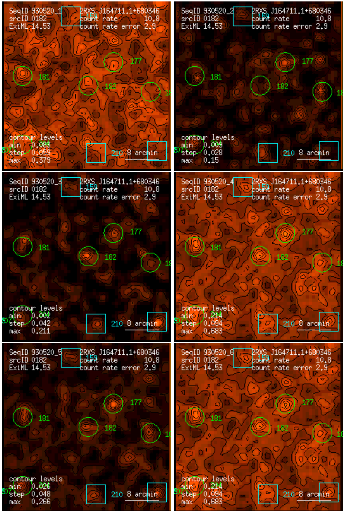
Figure 182: RASS 930520: detection 0182: band rate images, Gaussian filter: (1) PSPC channels 11 – 41, (2) 52 – 90, (3) 91 – 201, (4) 11 – 235, (5) 52 – 201, (6) 11 – 201. Broad band rates in counts/ks. Band rate contour levels in counts/ks/arcmin 2 .
