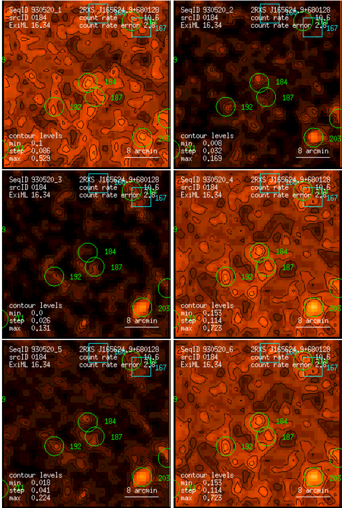
Figure 184: RASS 930520: detection 0184: band rate images, Gaussian filter: (1) PSPC channels 11 – 41, (2) 52 – 90, (3) 91 – 201, (4) 11 – 235, (5) 52 – 201, (6) 11 – 201. Broad band rates in counts/ks. Band rate contour levels in counts/ks/arcmin 2 .
