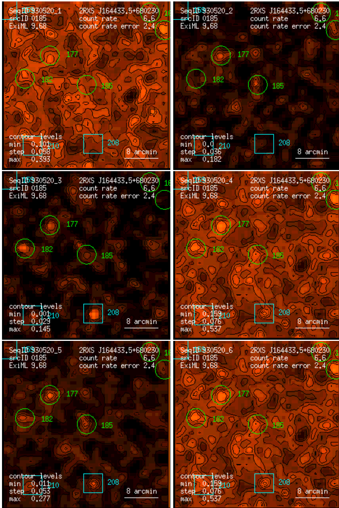
Figure 185: RASS 930520: detection 0185: band rate images, Gaussian filter: (1) PSPC channels 11 – 41, (2) 52 – 90, (3) 91 – 201, (4) 11 – 235, (5) 52 – 201, (6) 11 – 201. Broad band rates in counts/ks. Band rate contour levels in counts/ks/arcmin 2 .
