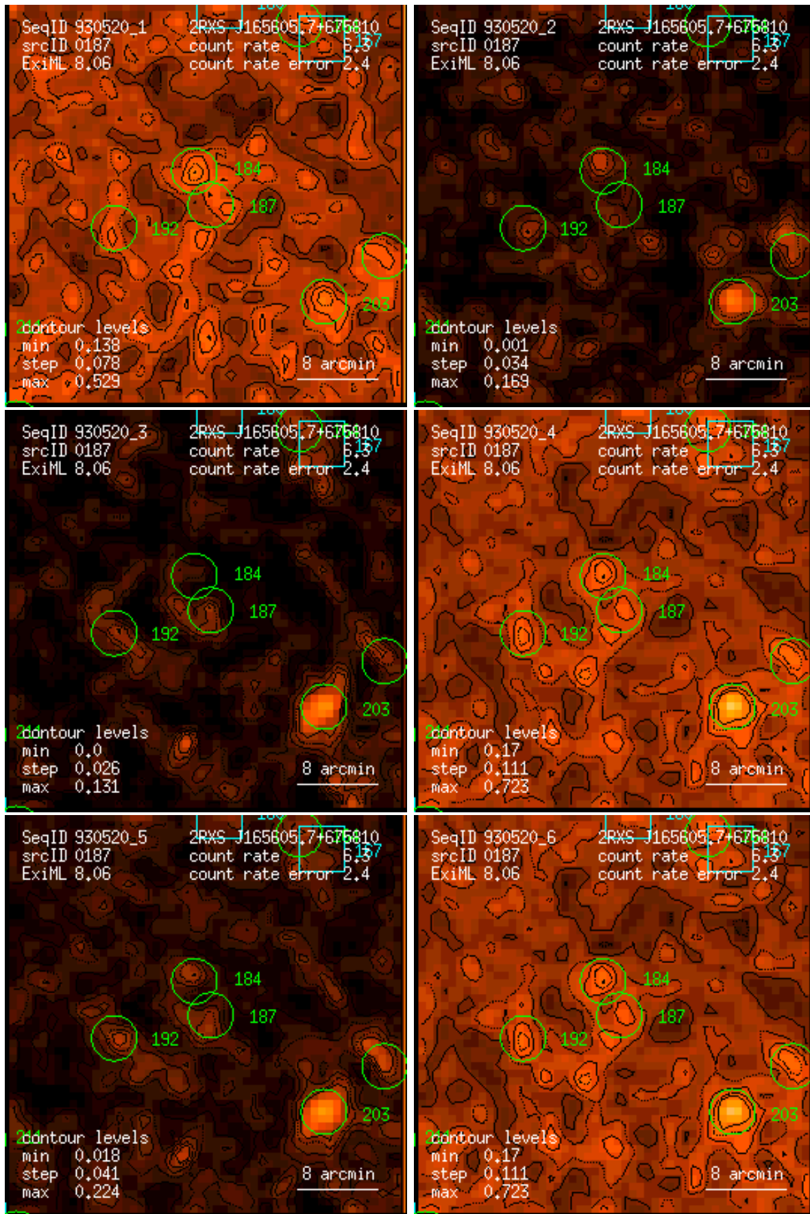
Figure 187: RASS 930520: detection 0187: band rate images, Gaussian filter: (1) PSPC channels 11 – 41, (2) 52 – 90, (3) 91 – 201, (4) 11 – 235, (5) 52 – 201, (6) 11 – 201. Broad band rates in counts/ks. Band rate contour levels in counts/ks/arcmin 2 .
