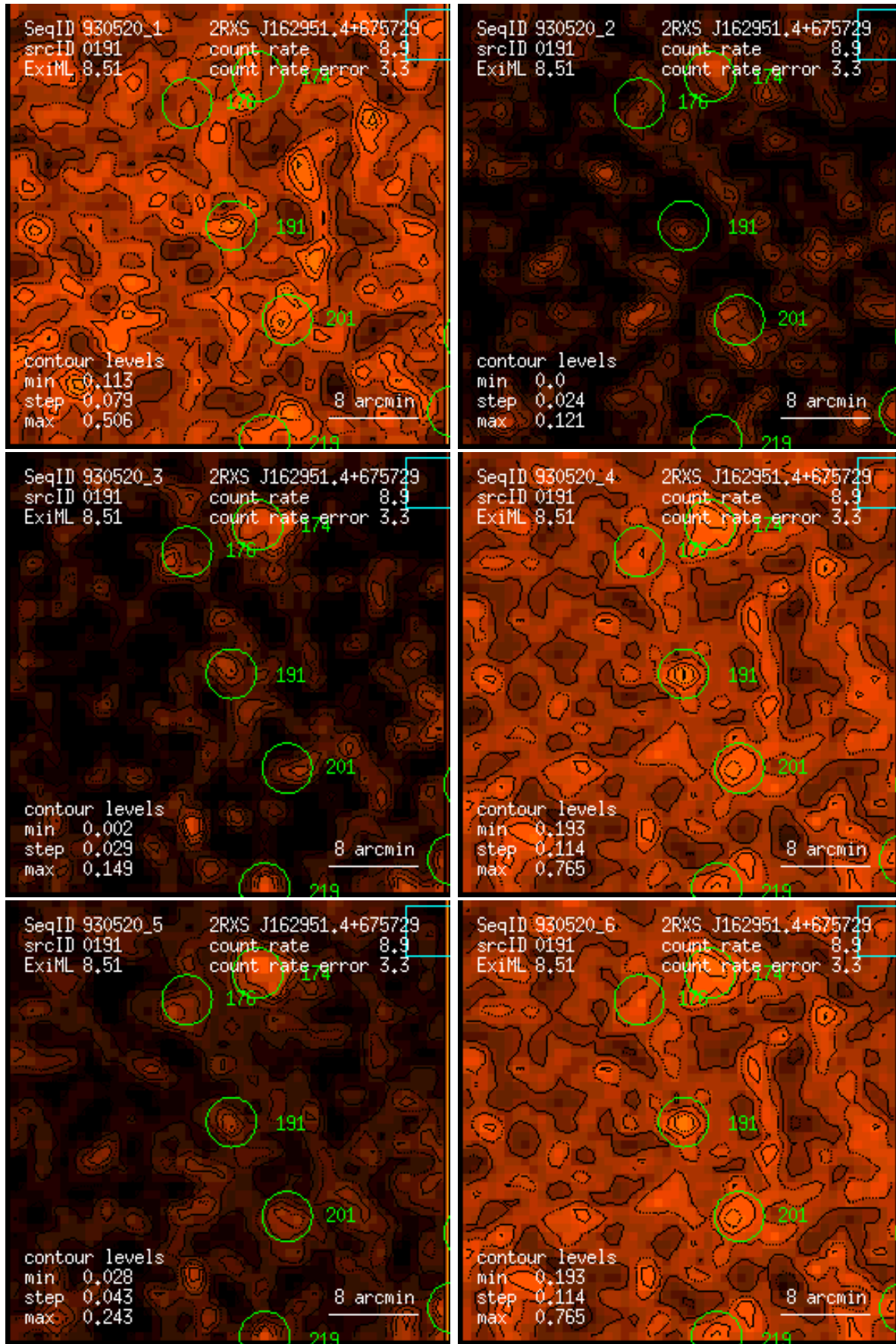
Figure 191: RASS 930520: detection 0191: band rate images, Gaussian filter: (1) PSPC channels 11 – 41, (2) 52 – 90, (3) 91 – 201, (4) 11 – 235, (5) 52 – 201, (6) 11 – 201. Broad band rates in counts/ks. Band rate contour levels in counts/ks/arcmin 2 .
