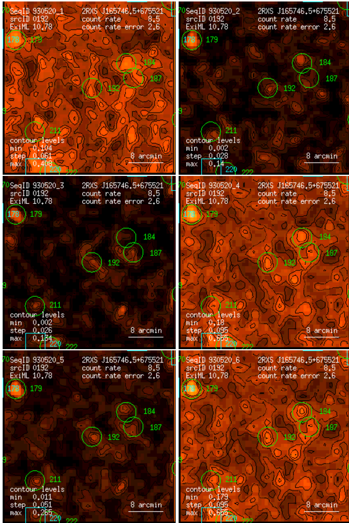
Figure 192: RASS 930520: detection 0192: band rate images, Gaussian filter: (1) PSPC channels 11 – 41, (2) 52 – 90, (3) 91 – 201, (4) 11 – 235, (5) 52 – 201, (6) 11 – 201. Broad band rates in counts/ks. Band rate contour levels in counts/ks/arcmin 2 .
