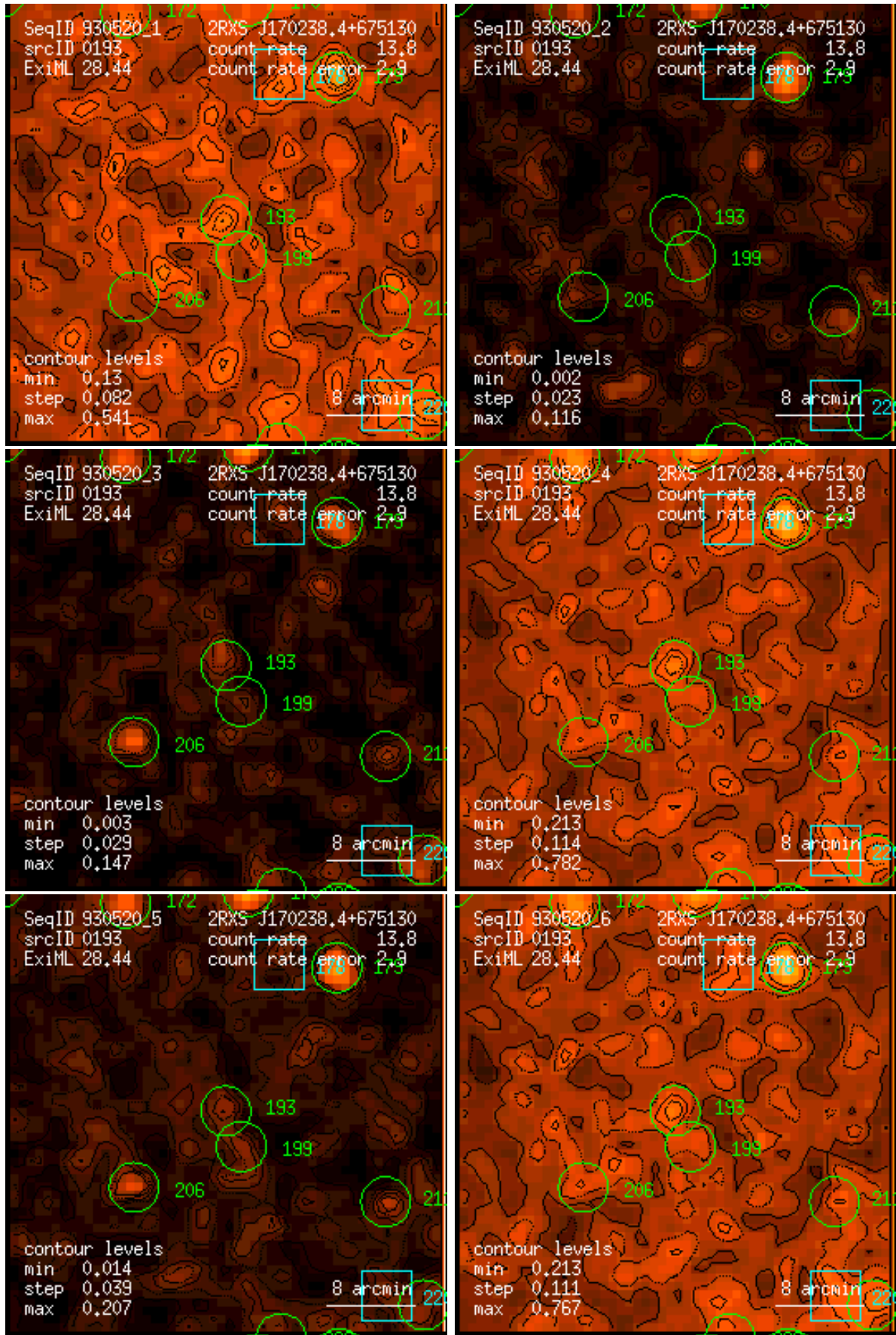
Figure 193: RASS 930520: detection 0193: band rate images, Gaussian filter: (1) PSPC channels 11 – 41, (2) 52 – 90, (3) 91 – 201, (4) 11 – 235, (5) 52 – 201, (6) 11 – 201. Broad band rates in counts/ks. Band rate contour levels in counts/ks/arcmin 2 .
