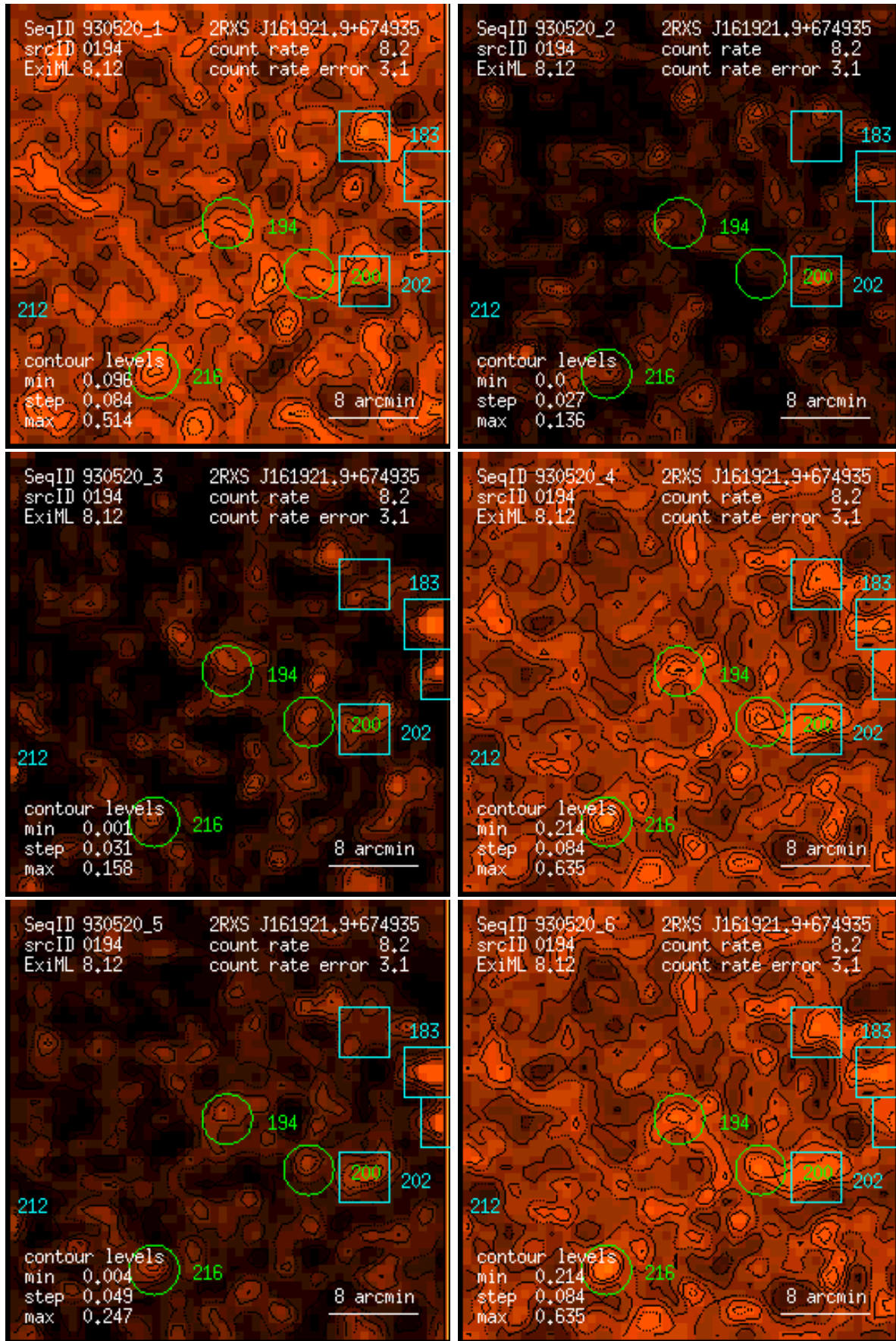
Figure 194: RASS 930520: detection 0194: band rate images, Gaussian filter: (1) PSPC channels 11 – 41, (2) 52 – 90, (3) 91 – 201, (4) 11 – 235, (5) 52 – 201, (6) 11 – 201. Broad band rates in counts/ks. Band rate contour levels in counts/ks/arcmin 2 .
