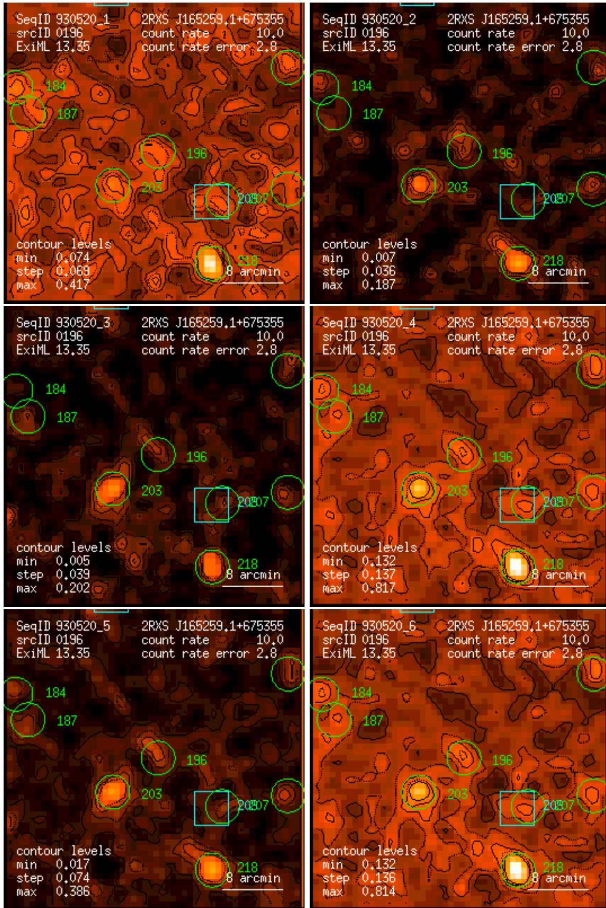
Figure 196: RASS 930520: detection 0196: band rate images, Gaussian filter: (1) PSPC channels 11 – 41, (2) 52 – 90, (3) 91 – 201, (4) 11 – 235, (5) 52 – 201, (6) 11 – 201. Broad band rates in counts/ks. Band rate contour levels in counts/ks/arcmin 2 .
