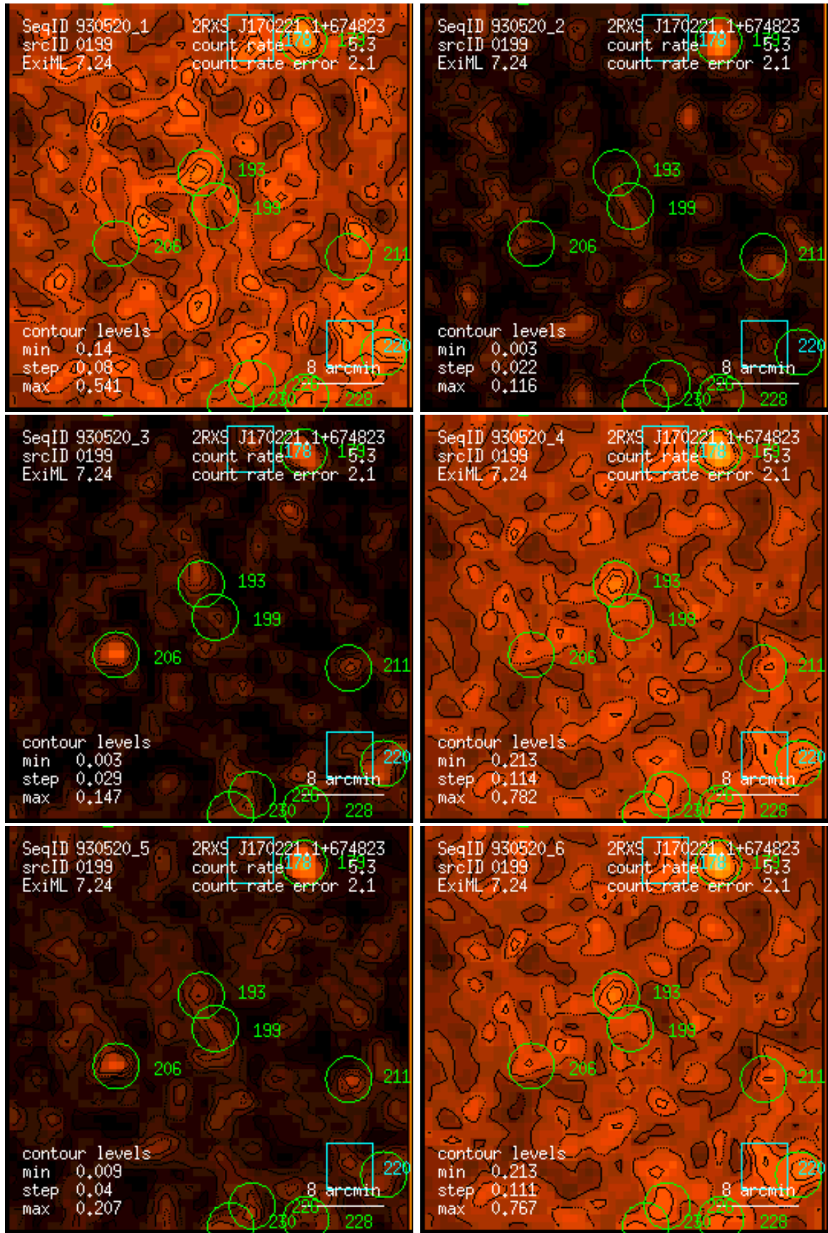
Figure 199: RASS 930520: detection 0199: band rate images, Gaussian filter: (1) PSPC channels 11 – 41, (2) 52 – 90, (3) 91 – 201, (4) 11 – 235, (5) 52 – 201, (6) 11 – 201. Broad band rates in counts/ks. Band rate contour levels in counts/ks/arcmin 2 .
