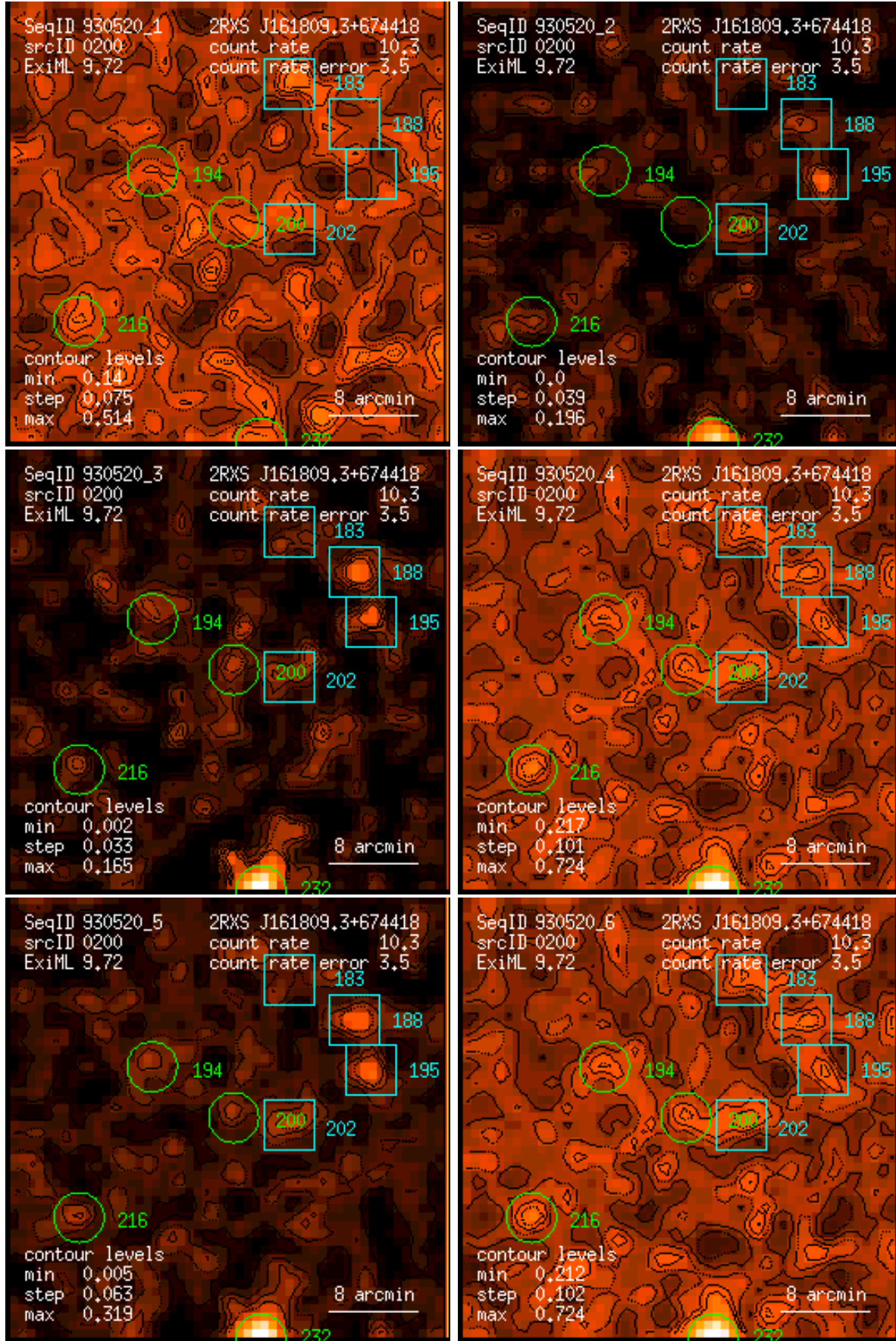
Figure 200: RASS 930520: detection 0200: band rate images, Gaussian filter: (1) PSPC channels 11 – 41, (2) 52 – 90, (3) 91 – 201, (4) 11 – 235, (5) 52 – 201, (6) 11 – 201. Broad band rates in counts/ks. Band rate contour levels in counts/ks/arcmin 2 .
