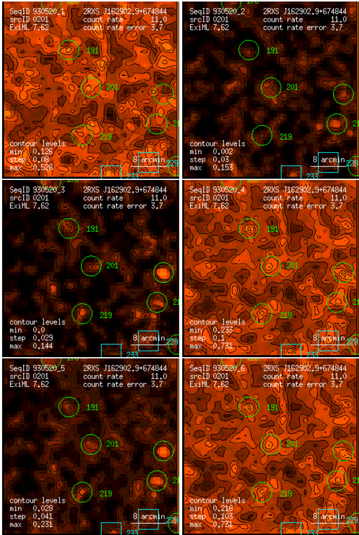
Figure 201: RASS 930520: detection 0201: band rate images, Gaussian filter: (1) PSPC channels 11 – 41, (2) 52 – 90, (3) 91 – 201, (4) 11 – 235, (5) 52 – 201, (6) 11 – 201. Broad band rates in counts/ks. Band rate contour levels in counts/ks/arcmin 2 .
