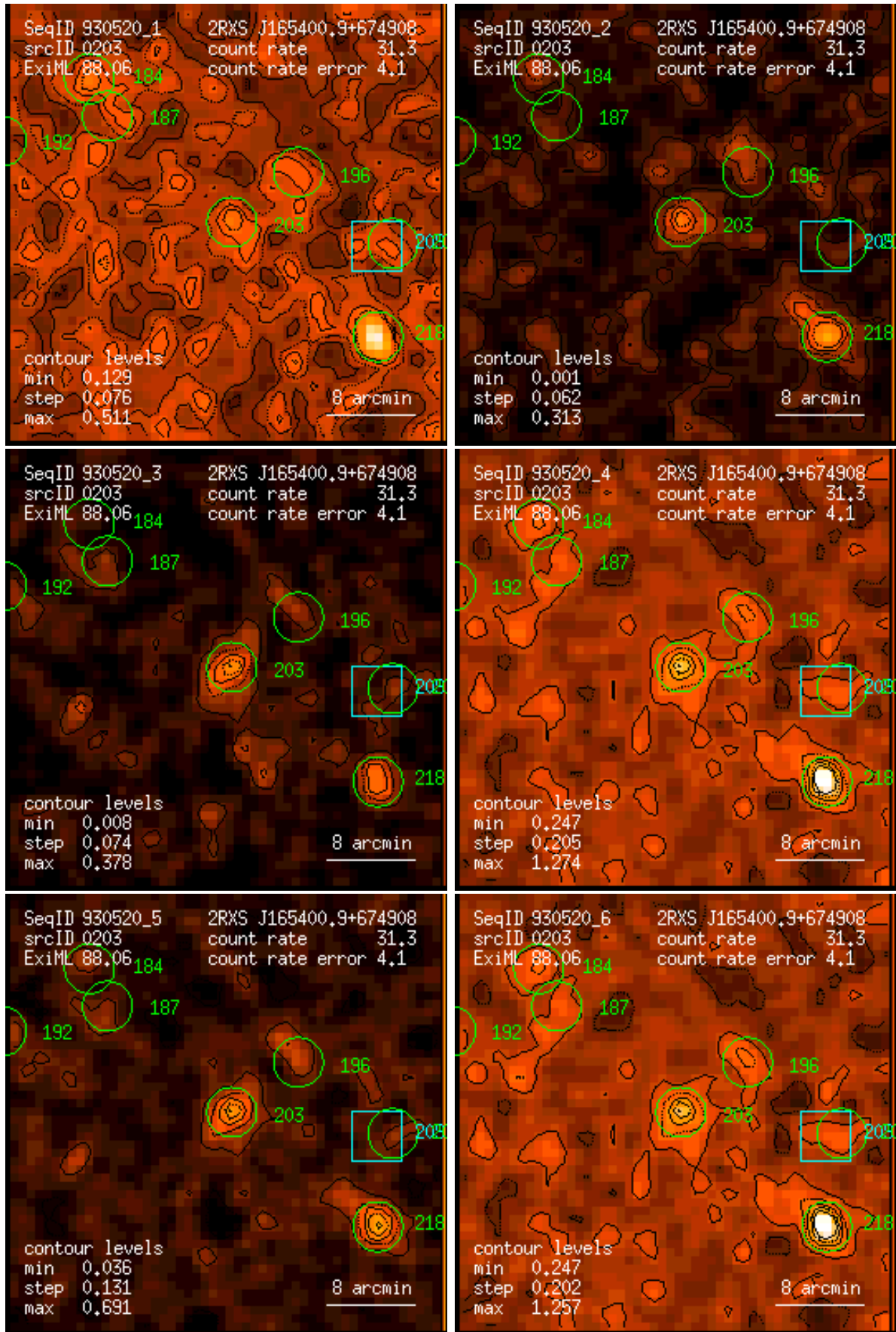
Figure 203: RASS 930520: detection 0203: band rate images, Gaussian filter: (1) PSPC channels 11 – 41, (2) 52 – 90, (3) 91 – 201, (4) 11 – 235, (5) 52 – 201, (6) 11 – 201. Broad band rates in counts/ks. Band rate contour levels in counts/ks/arcmin 2 .
