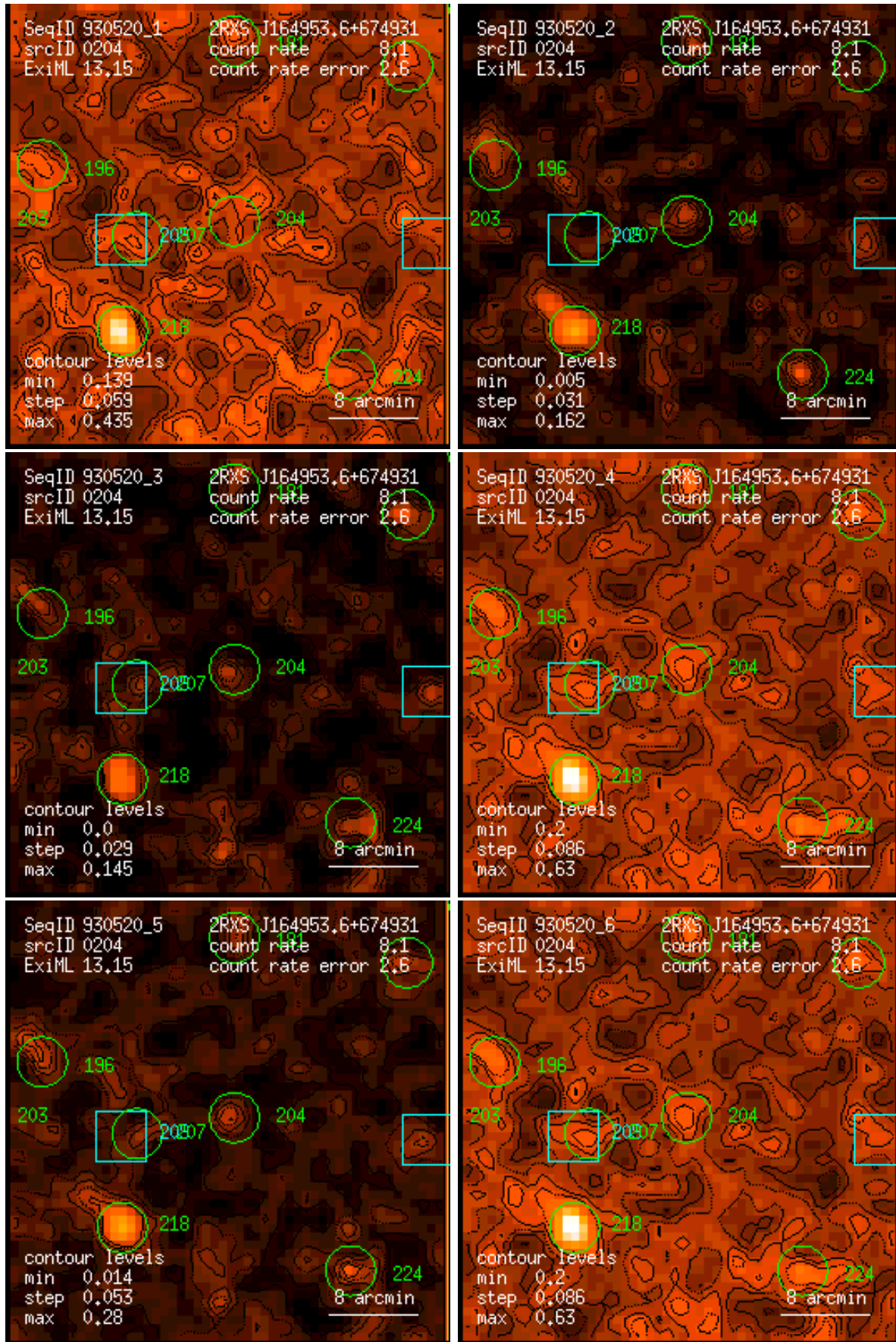
Figure 204: RASS 930520: detection 0204: band rate images, Gaussian filter: (1) PSPC channels 11 – 41, (2) 52 – 90, (3) 91 – 201, (4) 11 – 235, (5) 52 – 201, (6) 11 – 201. Broad band rates in counts/ks. Band rate contour levels in counts/ks/arcmin 2 .
