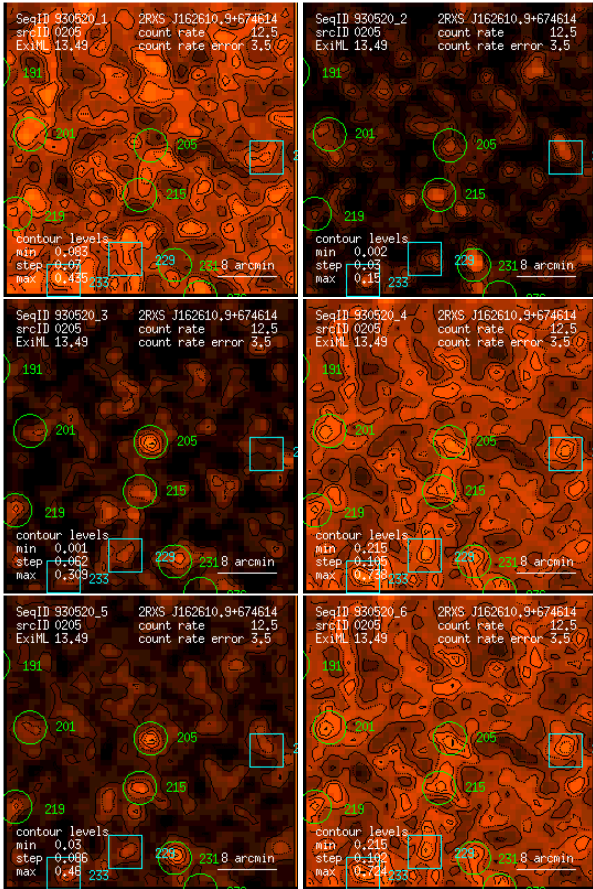
Figure 205: RASS 930520: detection 0205: band rate images, Gaussian filter: (1) PSPC channels 11 – 41, (2) 52 – 90, (3) 91 – 201, (4) 11 – 235, (5) 52 – 201, (6) 11 – 201. Broad band rates in counts/ks. Band rate contour levels in counts/ks/arcmin 2 .
