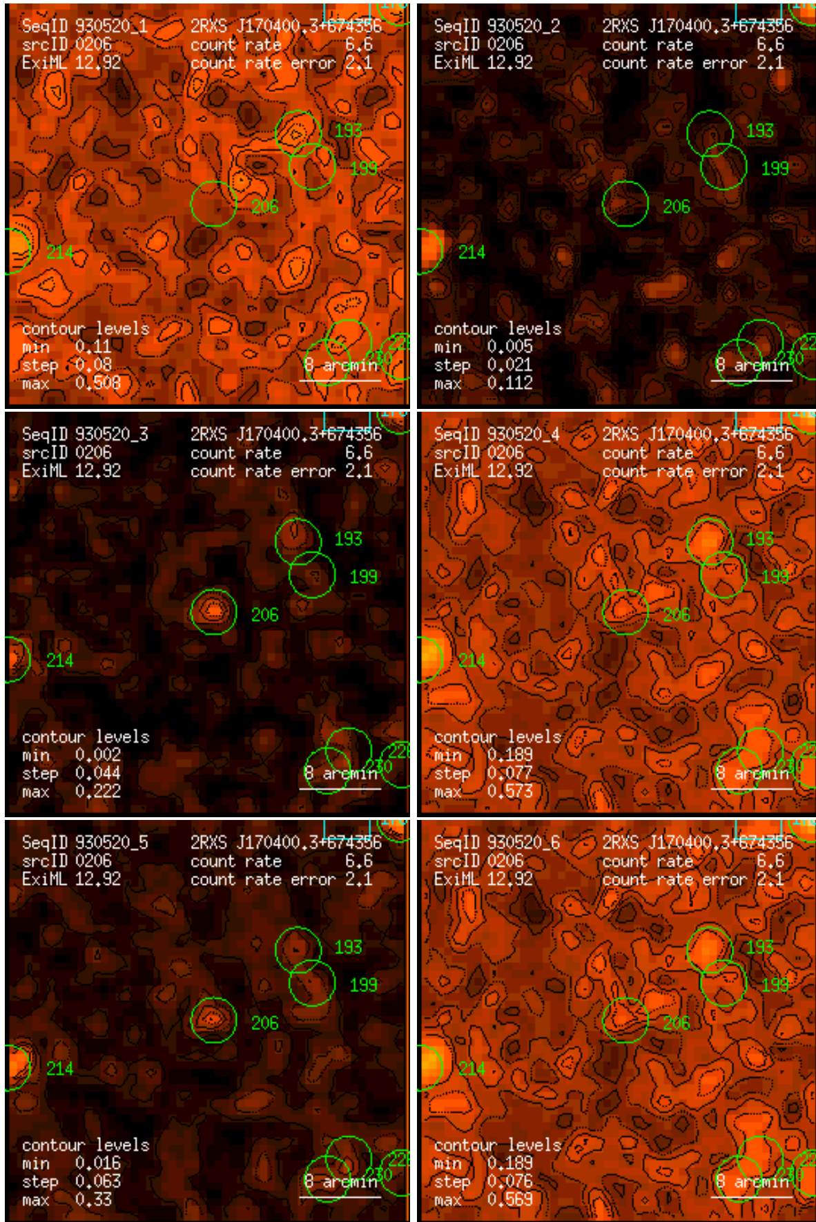
Figure 206: RASS 930520: detection 0206: band rate images, Gaussian filter: (1) PSPC channels 11 – 41, (2) 52 – 90, (3) 91 – 201, (4) 11 – 235, (5) 52 – 201, (6) 11 – 201. Broad band rates in counts/ks. Band rate contour levels in counts/ks/arcmin 2 .
