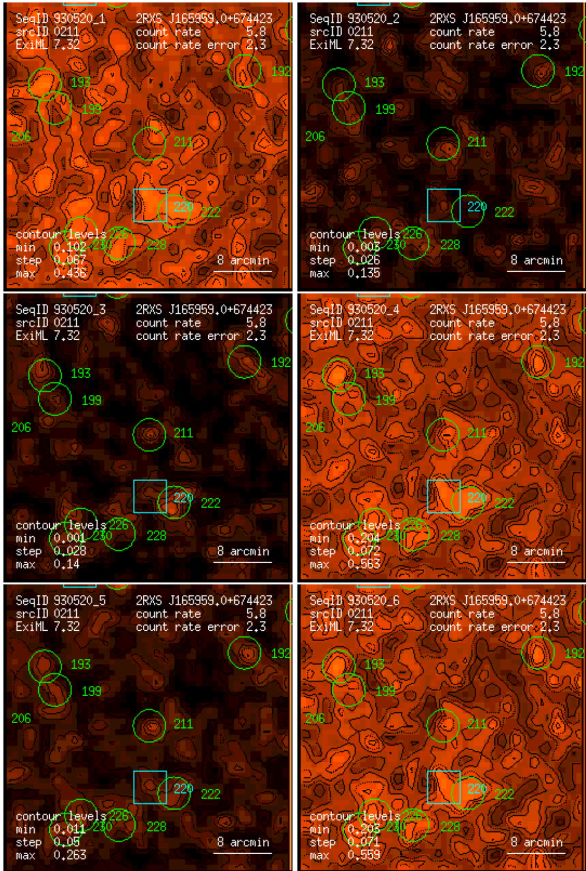
Figure 211: RASS 930520: detection 0211: band rate images, Gaussian filter: (1) PSPC channels 11 – 41, (2) 52 – 90, (3) 91 – 201, (4) 11 – 235, (5) 52 – 201, (6) 11 – 201. Broad band rates in counts/ks. Band rate contour levels in counts/ks/arcmin 2 .
