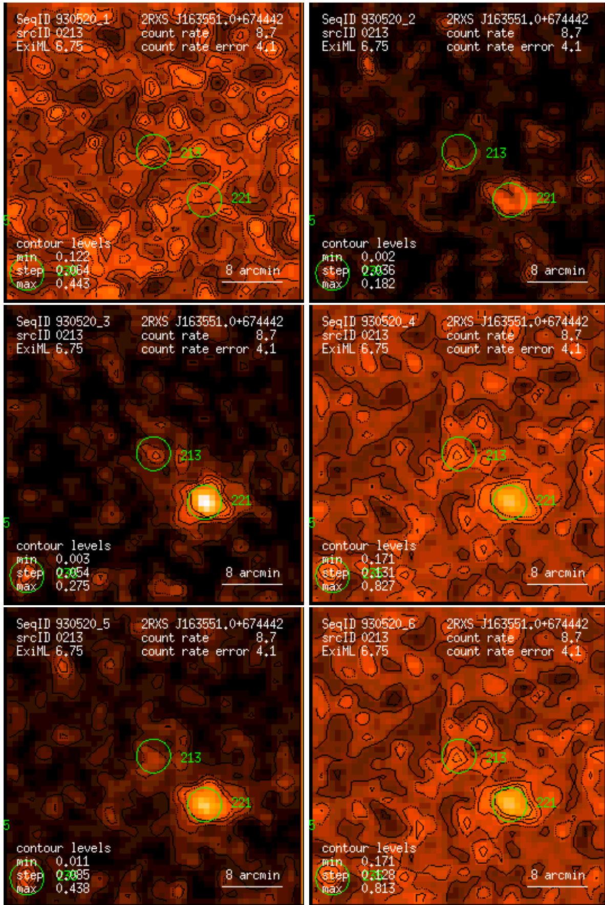
Figure 213: RASS 930520: detection 0213: band rate images, Gaussian filter: (1) PSPC channels 11 – 41, (2) 52 – 90, (3) 91 – 201, (4) 11 – 235, (5) 52 – 201, (6) 11 – 201. Broad band rates in counts/ks. Band rate contour levels in counts/ks/arcmin 2 .
