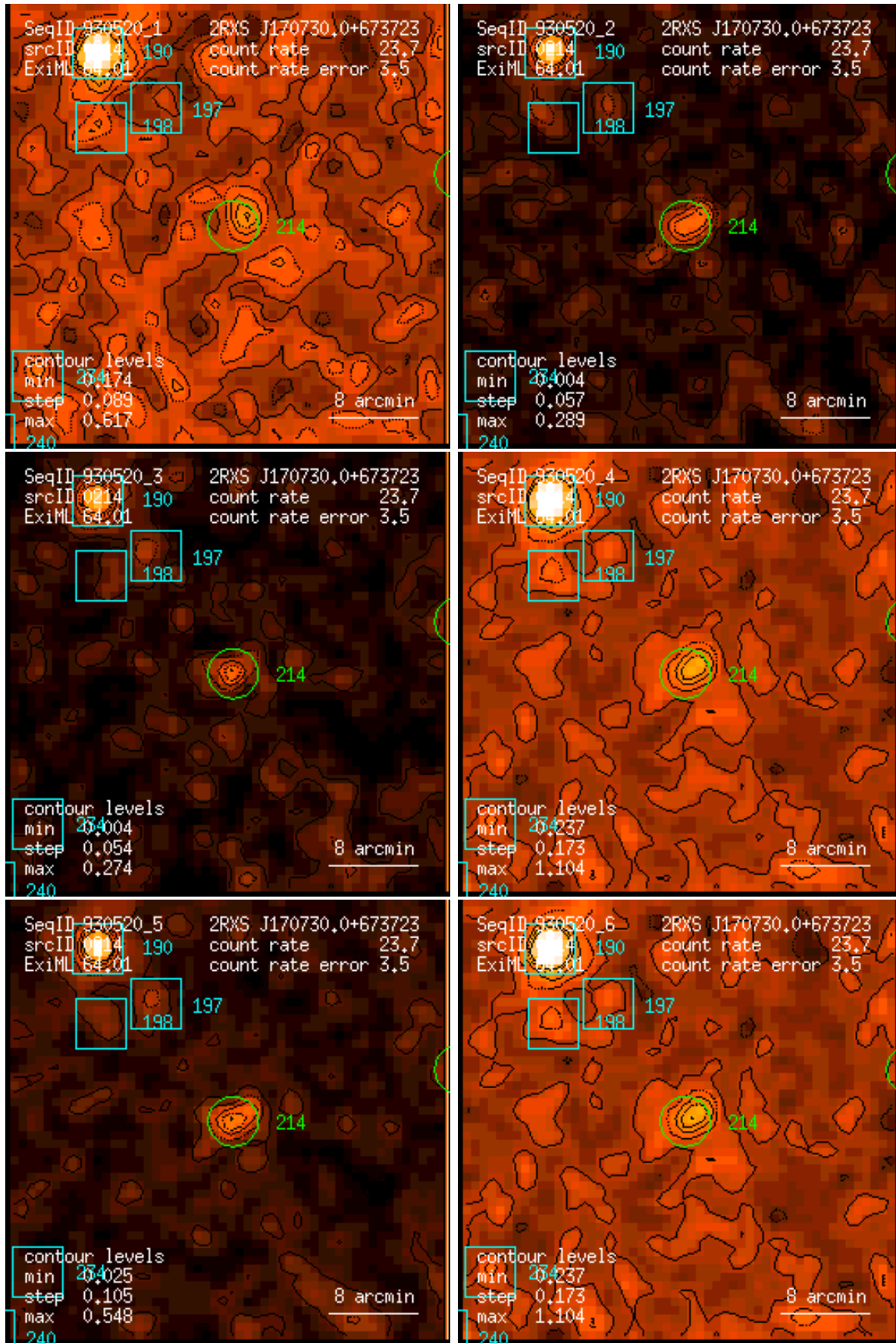
Figure 214: RASS 930520: detection 0214: band rate images, Gaussian filter: (1) PSPC channels 11 – 41, (2) 52 – 90, (3) 91 – 201, (4) 11 – 235, (5) 52 – 201, (6) 11 – 201. Broad band rates in counts/ks. Band rate contour levels in counts/ks/arcmin 2 .
