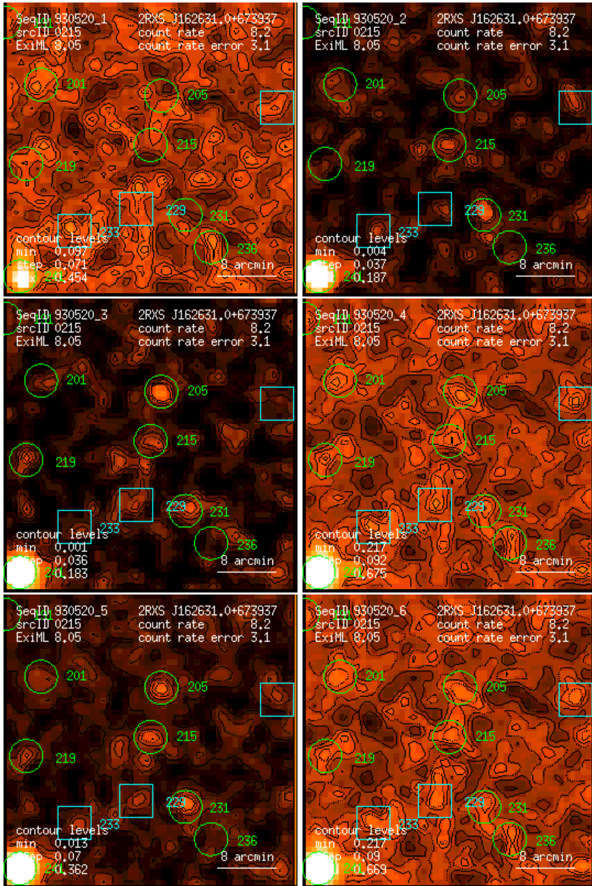
Figure 215: RASS 930520: detection 0215: band rate images, Gaussian filter: (1) PSPC channels 11 – 41, (2) 52 – 90, (3) 91 – 201, (4) 11 – 235, (5) 52 – 201, (6) 11 – 201. Broad band rates in counts/ks. Band rate contour levels in counts/ks/arcmin 2 .
