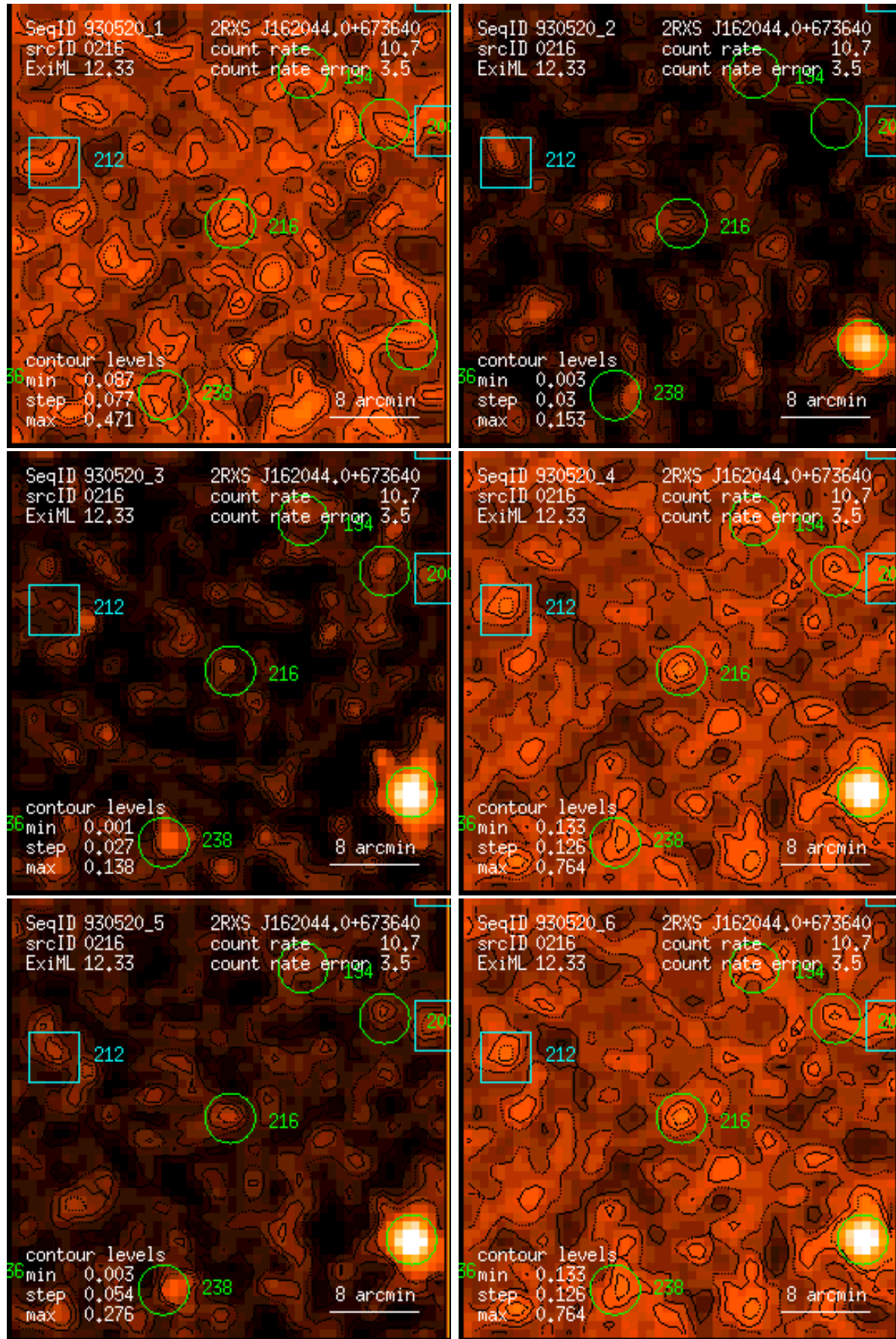
Figure 216: RASS 930520: detection 0216: band rate images, Gaussian filter: (1) PSPC channels 11 – 41, (2) 52 – 90, (3) 91 – 201, (4) 11 – 235, (5) 52 – 201, (6) 11 – 201. Broad band rates in counts/ks. Band rate contour levels in counts/ks/arcmin 2 .
