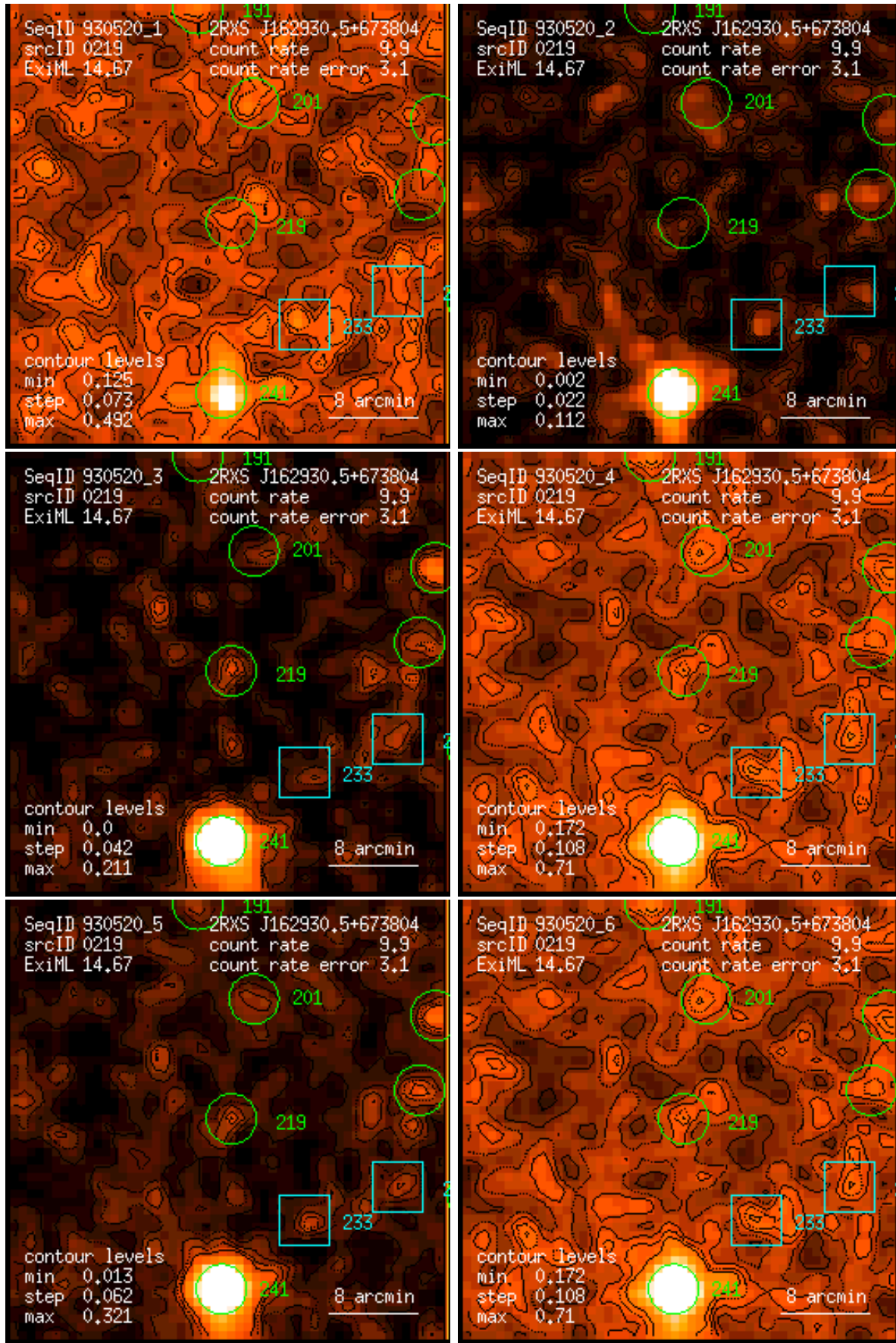
Figure 219: RASS 930520: detection 0219: band rate images, Gaussian filter: (1) PSPC channels 11 – 41, (2) 52 – 90, (3) 91 – 201, (4) 11 – 235, (5) 52 – 201, (6) 11 – 201. Broad band rates in counts/ks. Band rate contour levels in counts/ks/arcmin 2 .
