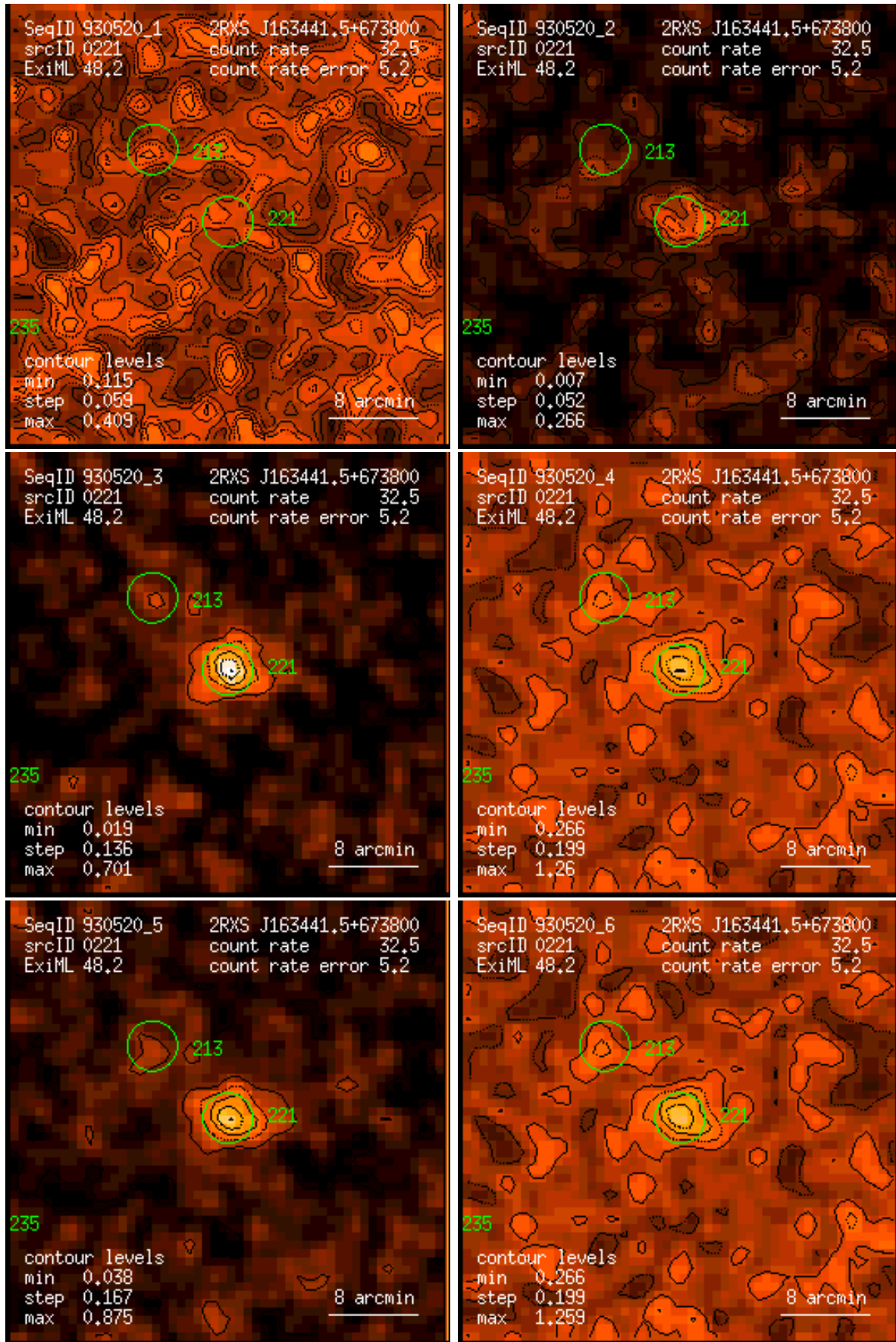
Figure 221: RASS 930520: detection 0221: band rate images, Gaussian filter: (1) PSPC channels 11 – 41, (2) 52 – 90, (3) 91 – 201, (4) 11 – 235, (5) 52 – 201, (6) 11 – 201. Broad band rates in counts/ks. Band rate contour levels in counts/ks/arcmin 2 .
