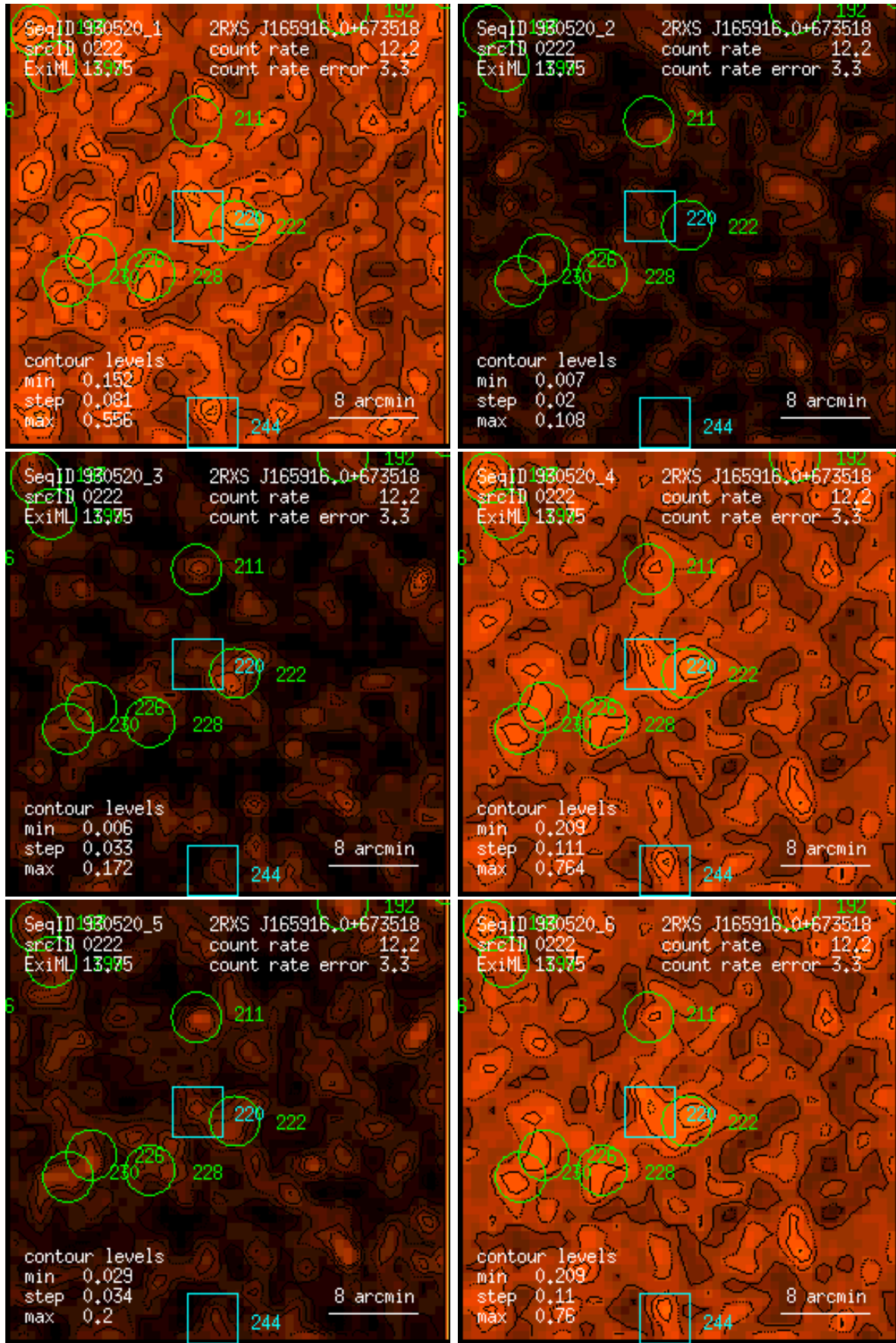
Figure 222: RASS 930520: detection 0222: band rate images, Gaussian filter: (1) PSPC channels 11 – 41, (2) 52 – 90, (3) 91 – 201, (4) 11 – 235, (5) 52 – 201, (6) 11 – 201. Broad band rates in counts/ks. Band rate contour levels in counts/ks/arcmin 2 .
