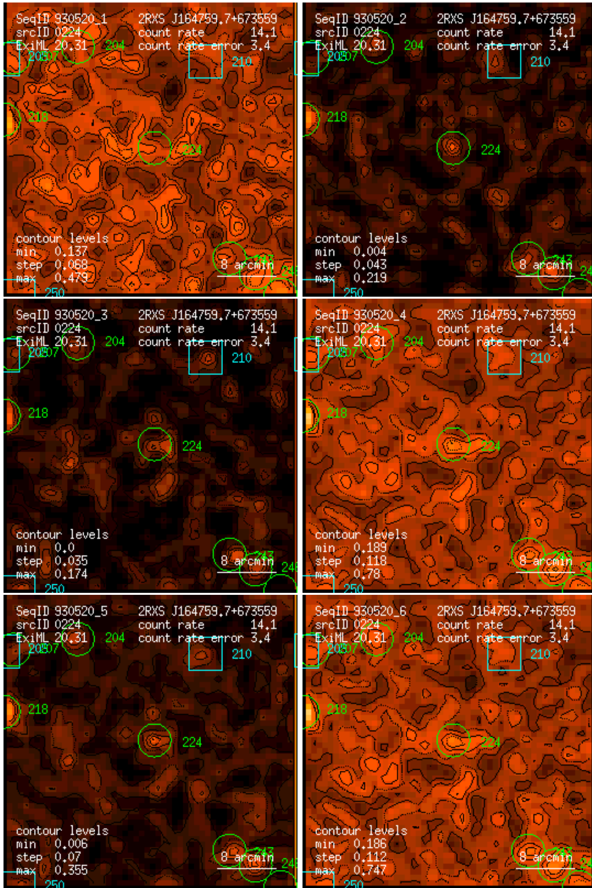
Figure 224: RASS 930520: detection 0224: band rate images, Gaussian filter: (1) PSPC channels 11 – 41, (2) 52 – 90, (3) 91 – 201, (4) 11 – 235, (5) 52 – 201, (6) 11 – 201. Broad band rates in counts/ks. Band rate contour levels in counts/ks/arcmin 2 .
