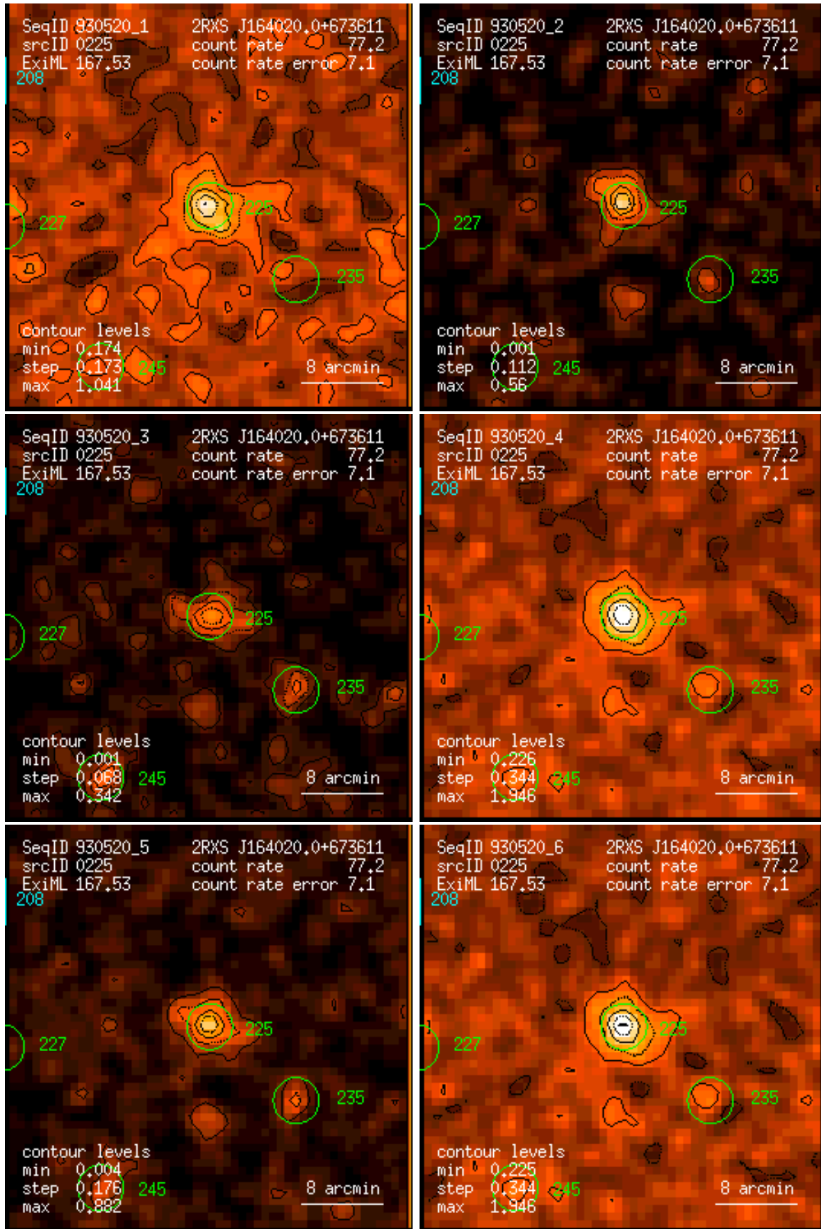
Figure 225: RASS 930520: detection 0225: band rate images, Gaussian filter: (1) PSPC channels 11 – 41, (2) 52 – 90, (3) 91 – 201, (4) 11 – 235, (5) 52 – 201, (6) 11 – 201. Broad band rates in counts/ks. Band rate contour levels in counts/ks/arcmin 2 .
