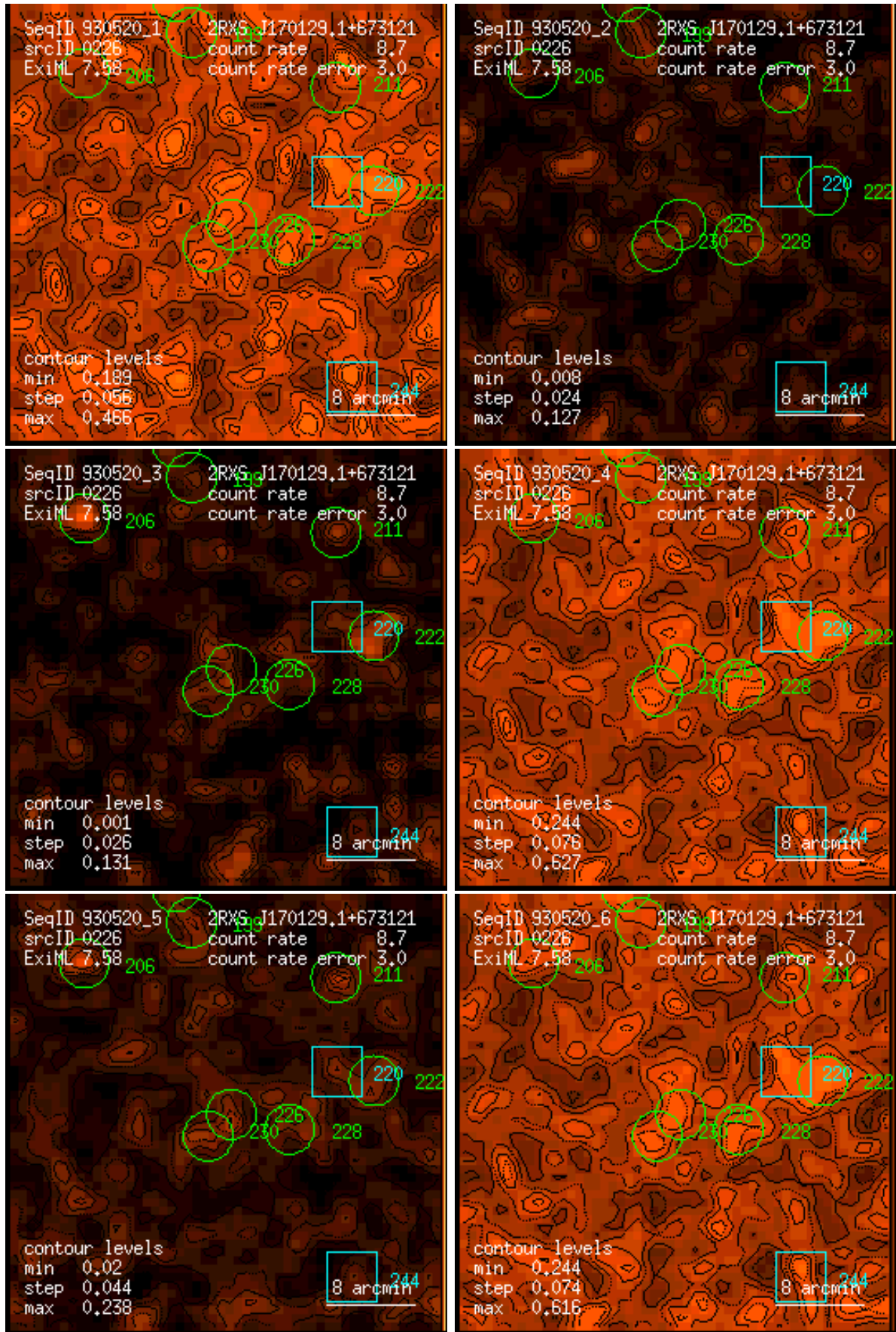
Figure 226: RASS 930520: detection 0226: band rate images, Gaussian filter: (1) PSPC channels 11 – 41, (2) 52 – 90, (3) 91 – 201, (4) 11 – 235, (5) 52 – 201, (6) 11 – 201. Broad band rates in counts/ks. Band rate contour levels in counts/ks/arcmin 2 .
