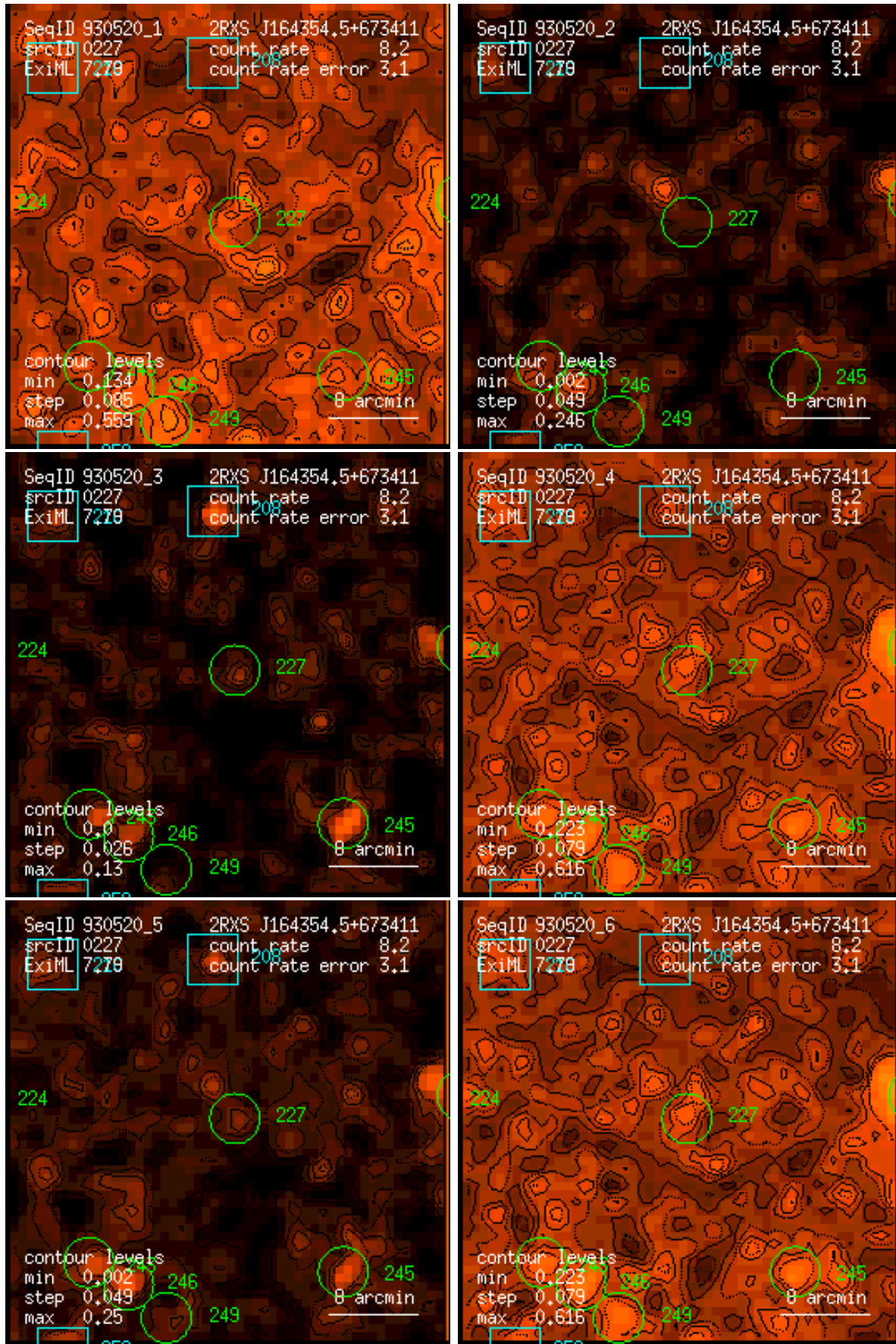
Figure 227: RASS 930520: detection 0227: band rate images, Gaussian filter: (1) PSPC channels 11 – 41, (2) 52 – 90, (3) 91 – 201, (4) 11 – 235, (5) 52 – 201, (6) 11 – 201. Broad band rates in counts/ks. Band rate contour levels in counts/ks/arcmin 2 .
