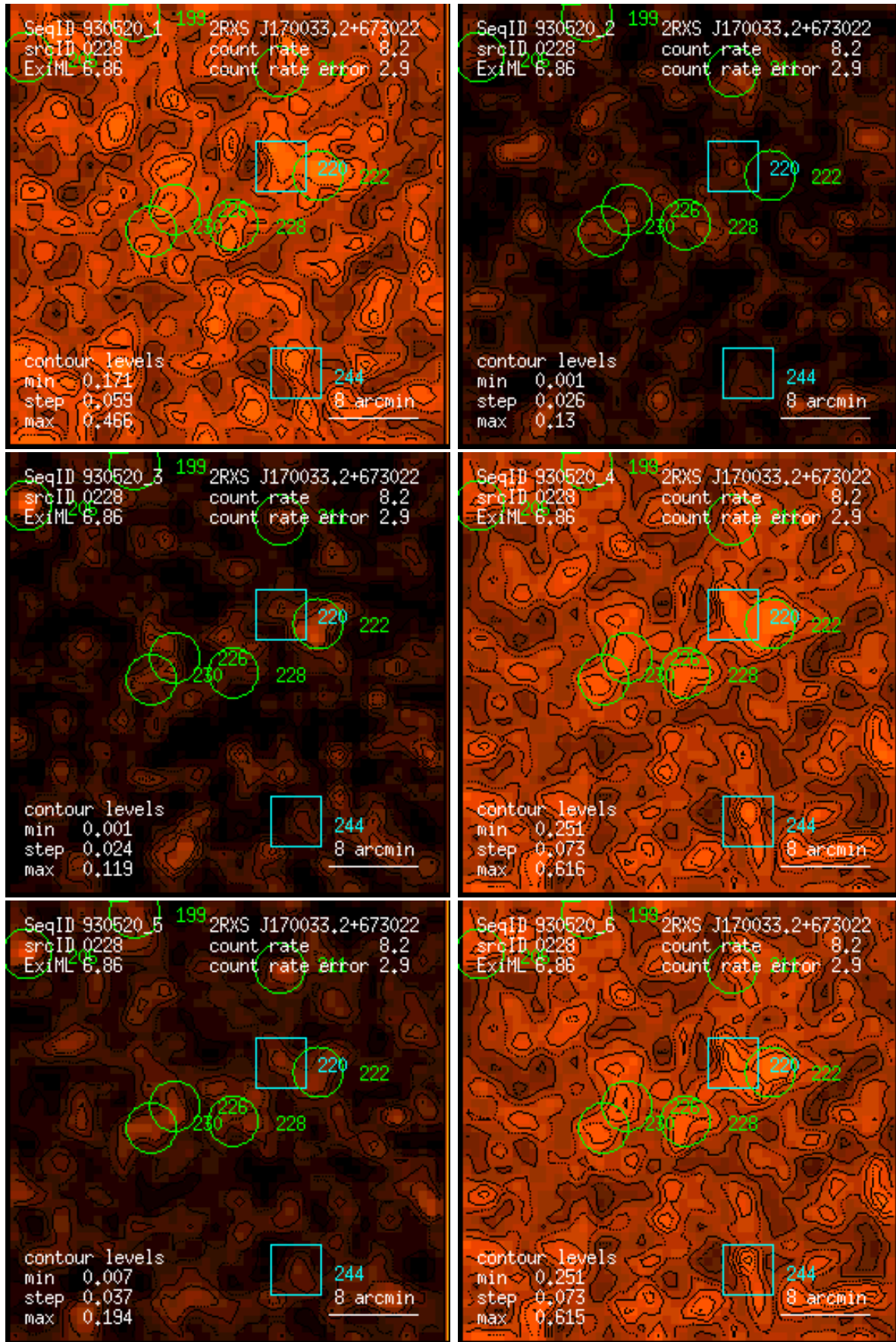
Figure 228: RASS 930520: detection 0228: band rate images, Gaussian filter: (1) PSPC channels 11 – 41, (2) 52 – 90, (3) 91 – 201, (4) 11 – 235, (5) 52 – 201, (6) 11 – 201. Broad band rates in counts/ks. Band rate contour levels in counts/ks/arcmin 2 .
