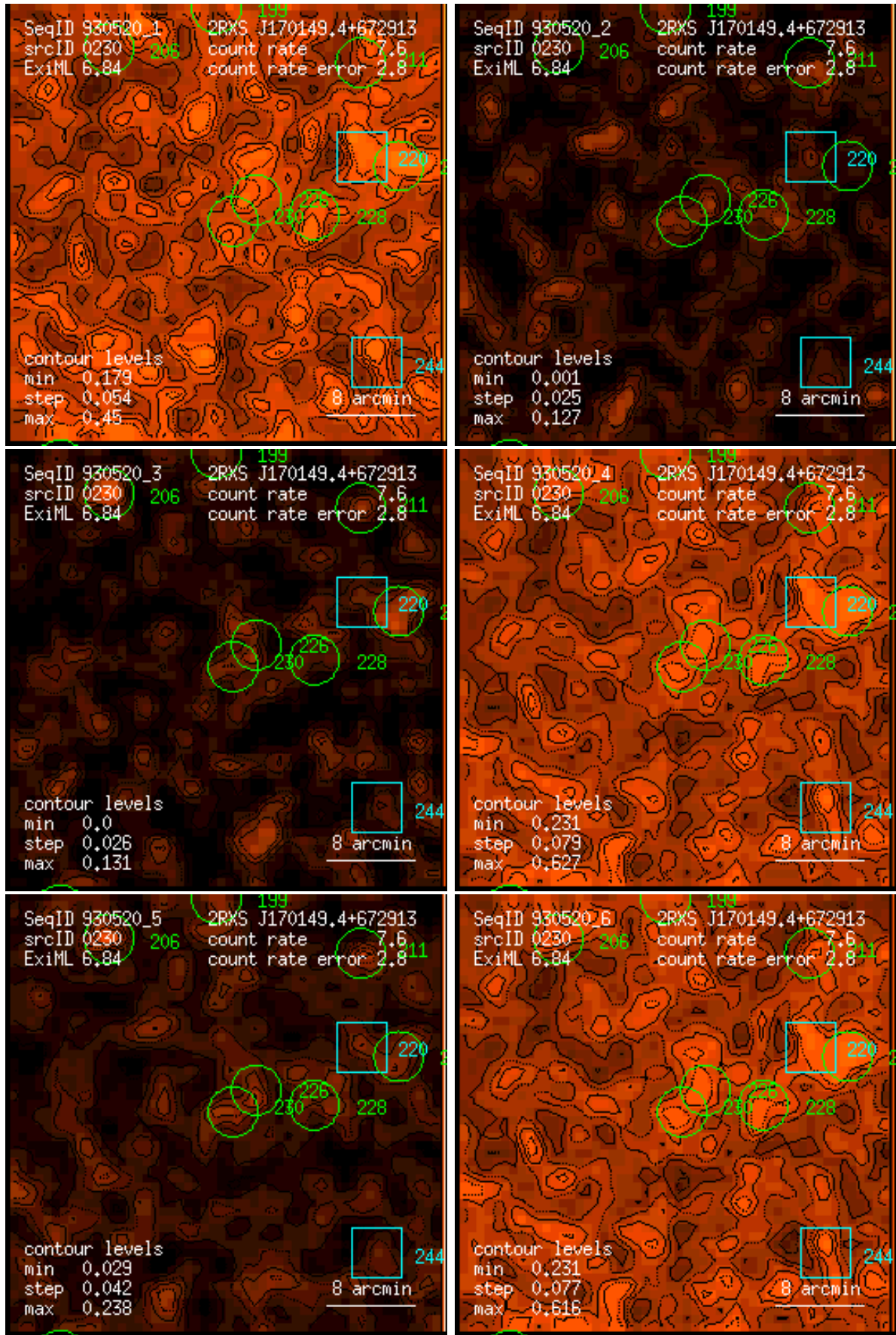
Figure 230: RASS 930520: detection 0230: band rate images, Gaussian filter: (1) PSPC channels 11 – 41, (2) 52 – 90, (3) 91 – 201, (4) 11 – 235, (5) 52 – 201, (6) 11 – 201. Broad band rates in counts/ks. Band rate contour levels in counts/ks/arcmin 2 .
