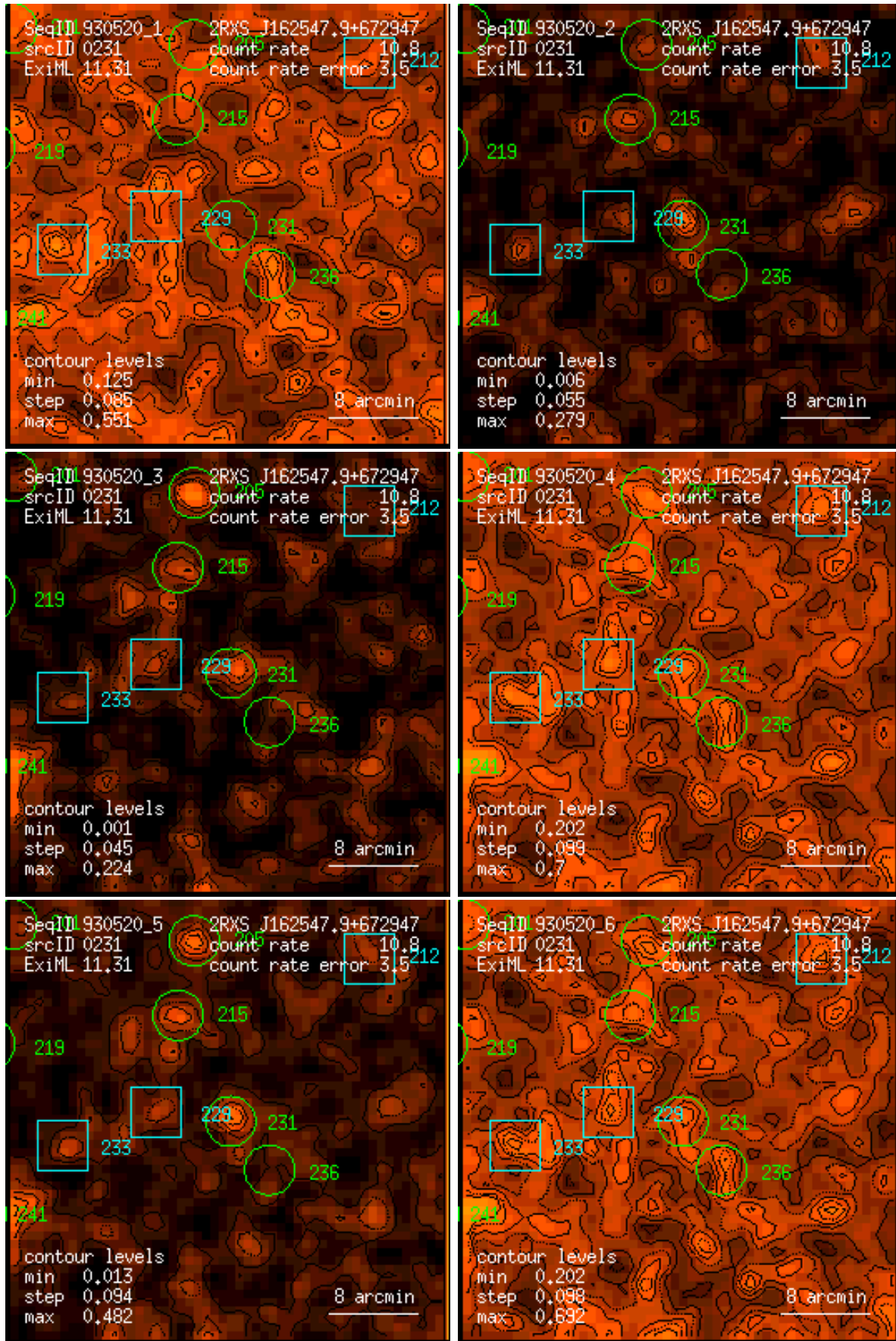
Figure 231: RASS 930520: detection 0231: band rate images, Gaussian filter: (1) PSPC channels 11 – 41, (2) 52 – 90, (3) 91 – 201, (4) 11 – 235, (5) 52 – 201, (6) 11 – 201. Broad band rates in counts/ks. Band rate contour levels in counts/ks/arcmin 2 .
