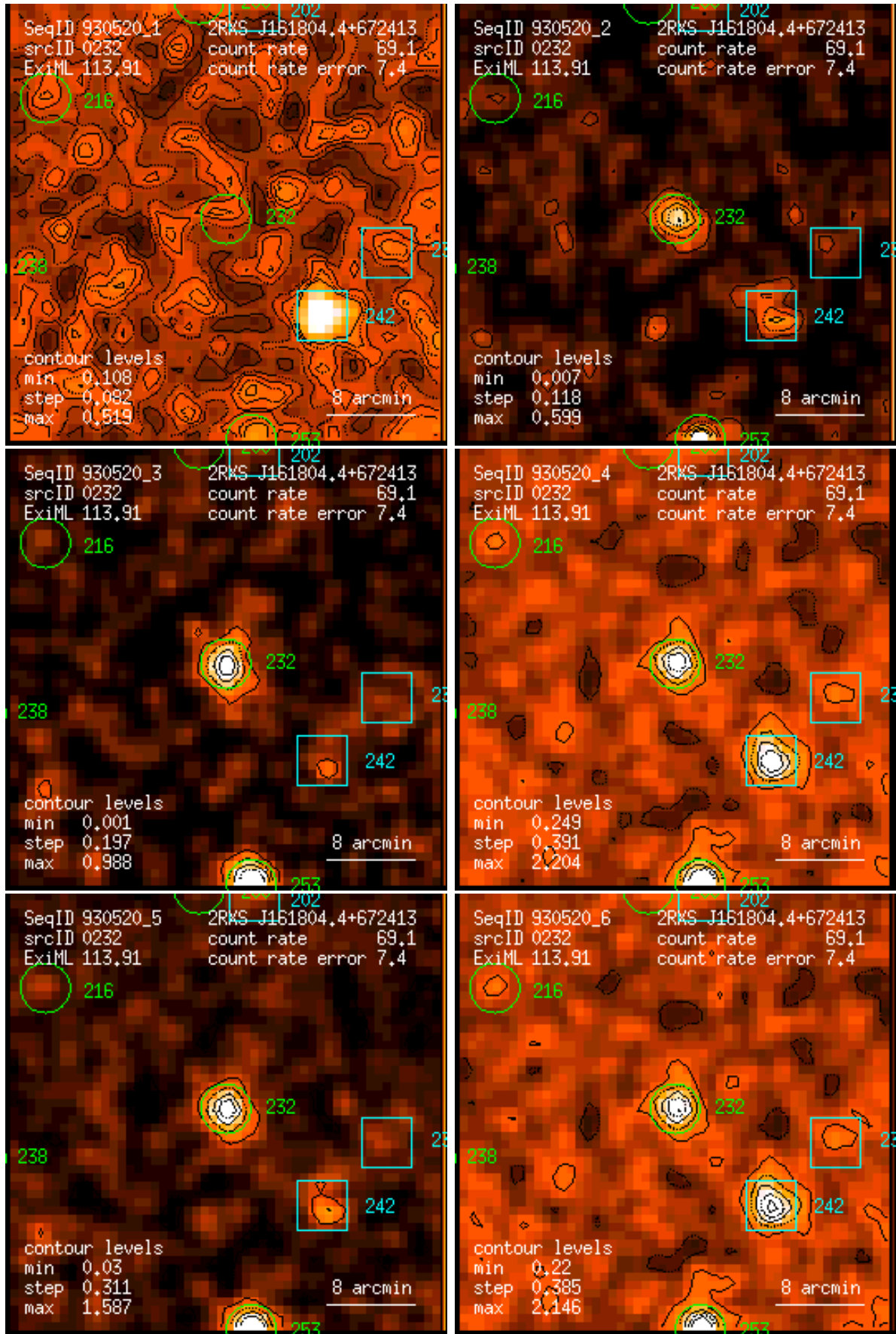
Figure 232: RASS 930520: detection 0232: band rate images, Gaussian filter: (1) PSPC channels 11 – 41, (2) 52 – 90, (3) 91 – 201, (4) 11 – 235, (5) 52 – 201, (6) 11 – 201. Broad band rates in counts/ks. Band rate contour levels in counts/ks/arcmin 2 .
