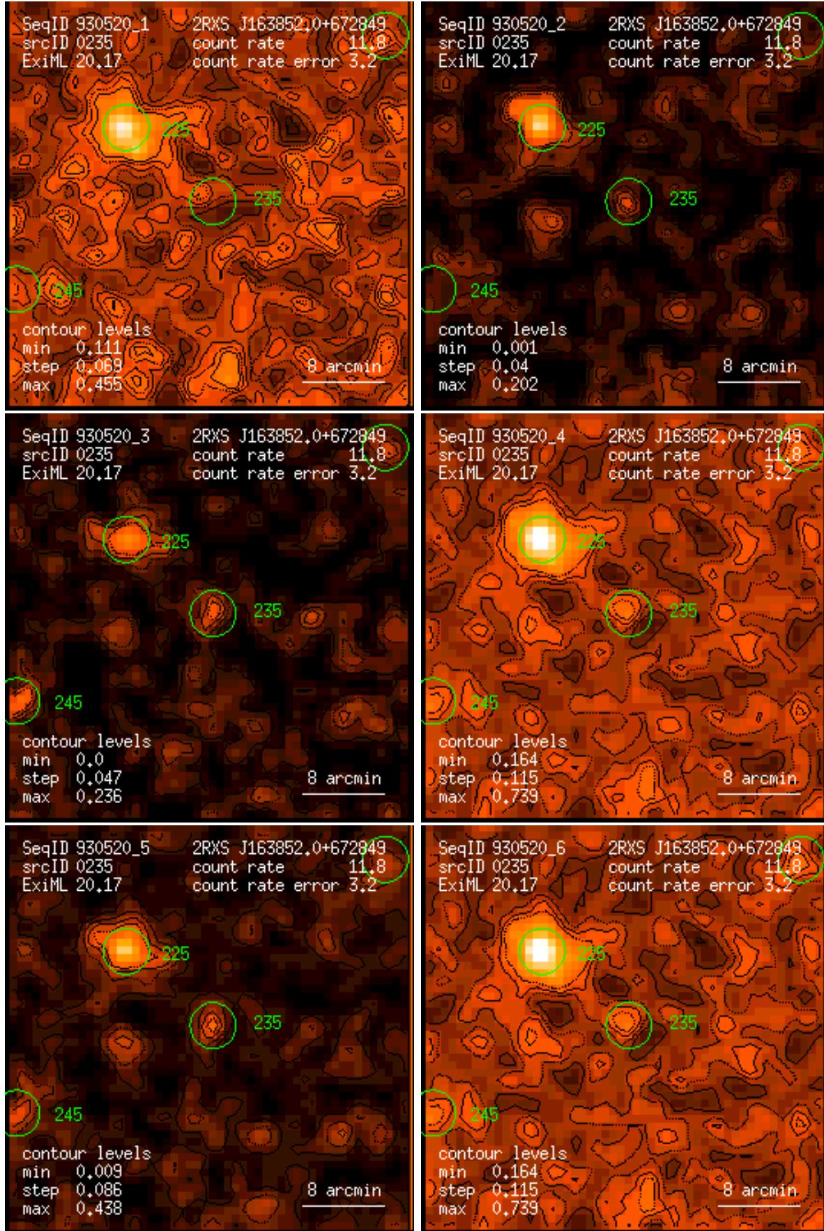
Figure 235: RASS 930520: detection 0235: band rate images, Gaussian filter: (1) PSPC channels 11 – 41, (2) 52 – 90, (3) 91 – 201, (4) 11 – 235, (5) 52 – 201, (6) 11 – 201. Broad band rates in counts/ks. Band rate contour levels in counts/ks/arcmin 2 .
