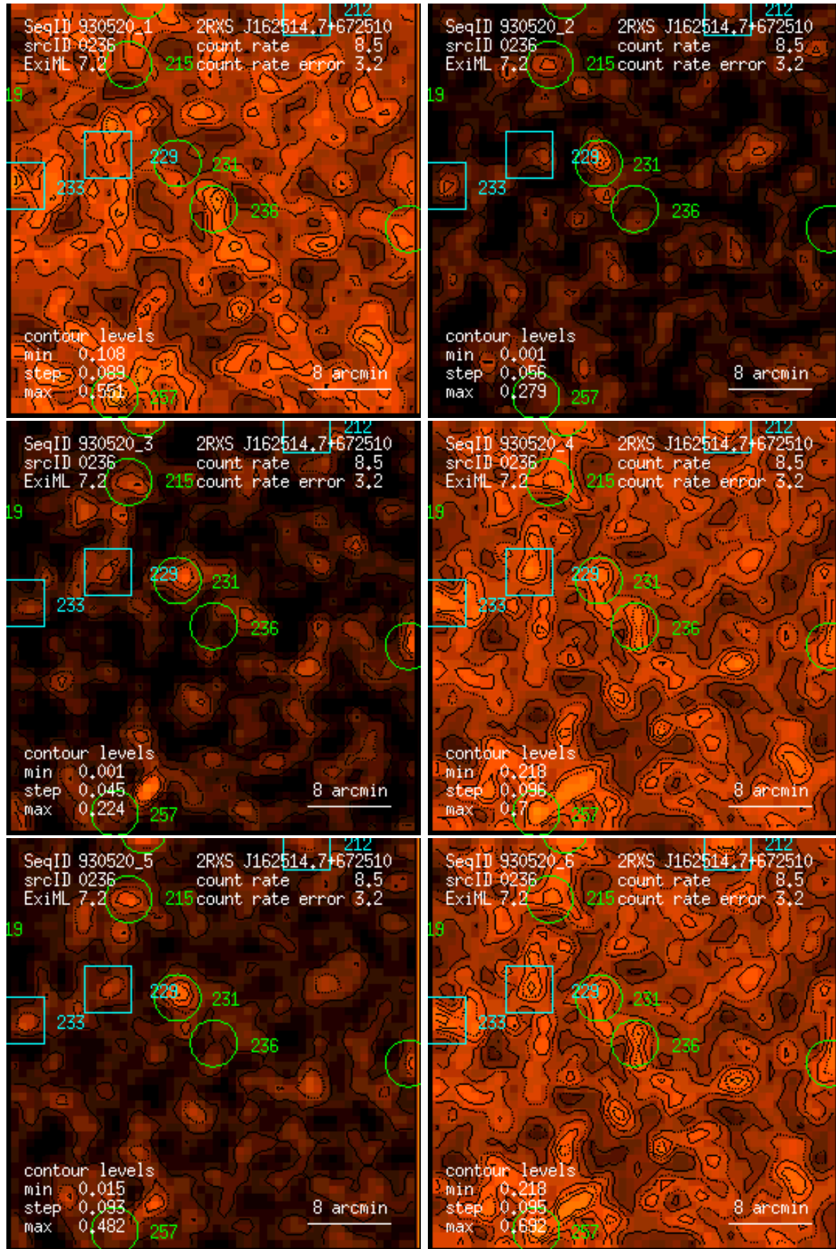
Figure 236: RASS 930520: detection 0236: band rate images, Gaussian filter: (1) PSPC channels 11 – 41, (2) 52 – 90, (3) 91 – 201, (4) 11 – 235, (5) 52 – 201, (6) 11 – 201. Broad band rates in counts/ks. Band rate contour levels in counts/ks/arcmin 2 .
